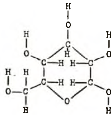
GLUCOSE
