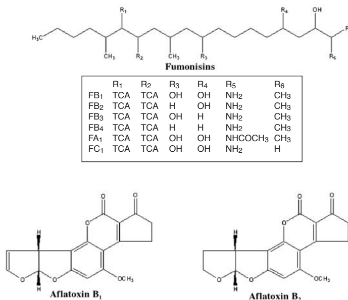
Figure 1. Chemical structures of aflatoxins B 1 and B 2 , and various fumonisin analogs. TCA = tricarballic acid (propane-1,2,3-tricarboxylic acid).
