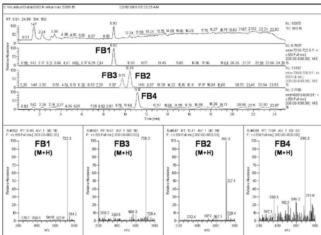
Figure 2. Chromatograms and mass spectra of various analogs of fumonisins (FB1, FB2, FB3, and FB4).
