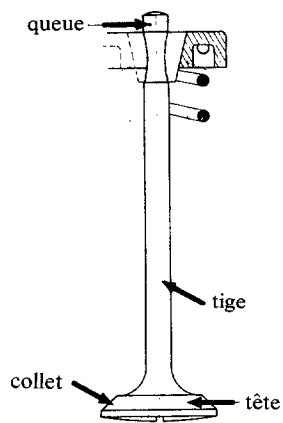
Soupape
