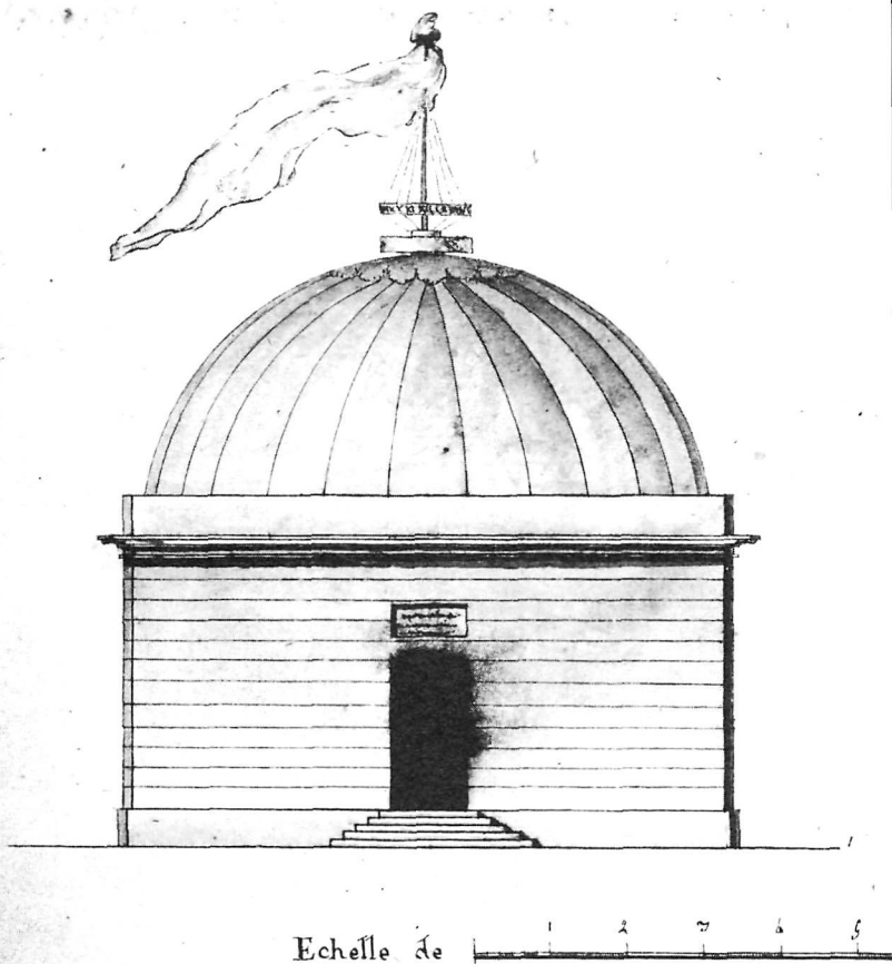
22 Belu, Elevation of a Temple Décadaire for a provincial town
