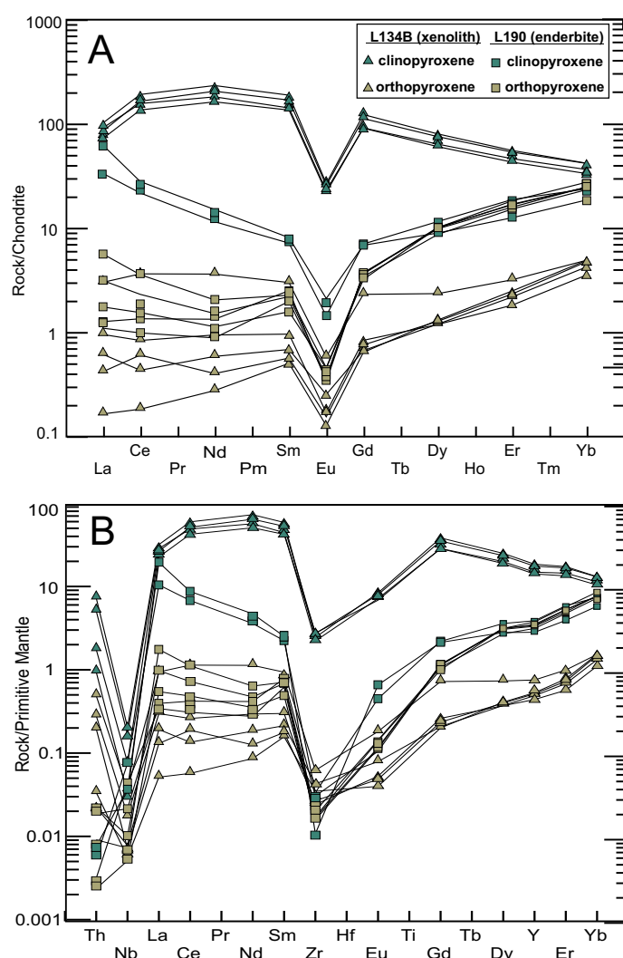
Figure 9. A) Chondrite-normalized REE plot (normalizing values taken from Sun and McDonough 1989) for orthopyroxene and clinopyroxene in enderbite intrusion and websterite xenolith. B) Primitive mantle-normalized extended trace element diagram (primitive mantle-normalizing values taken from Sun and McDonough 1989).
