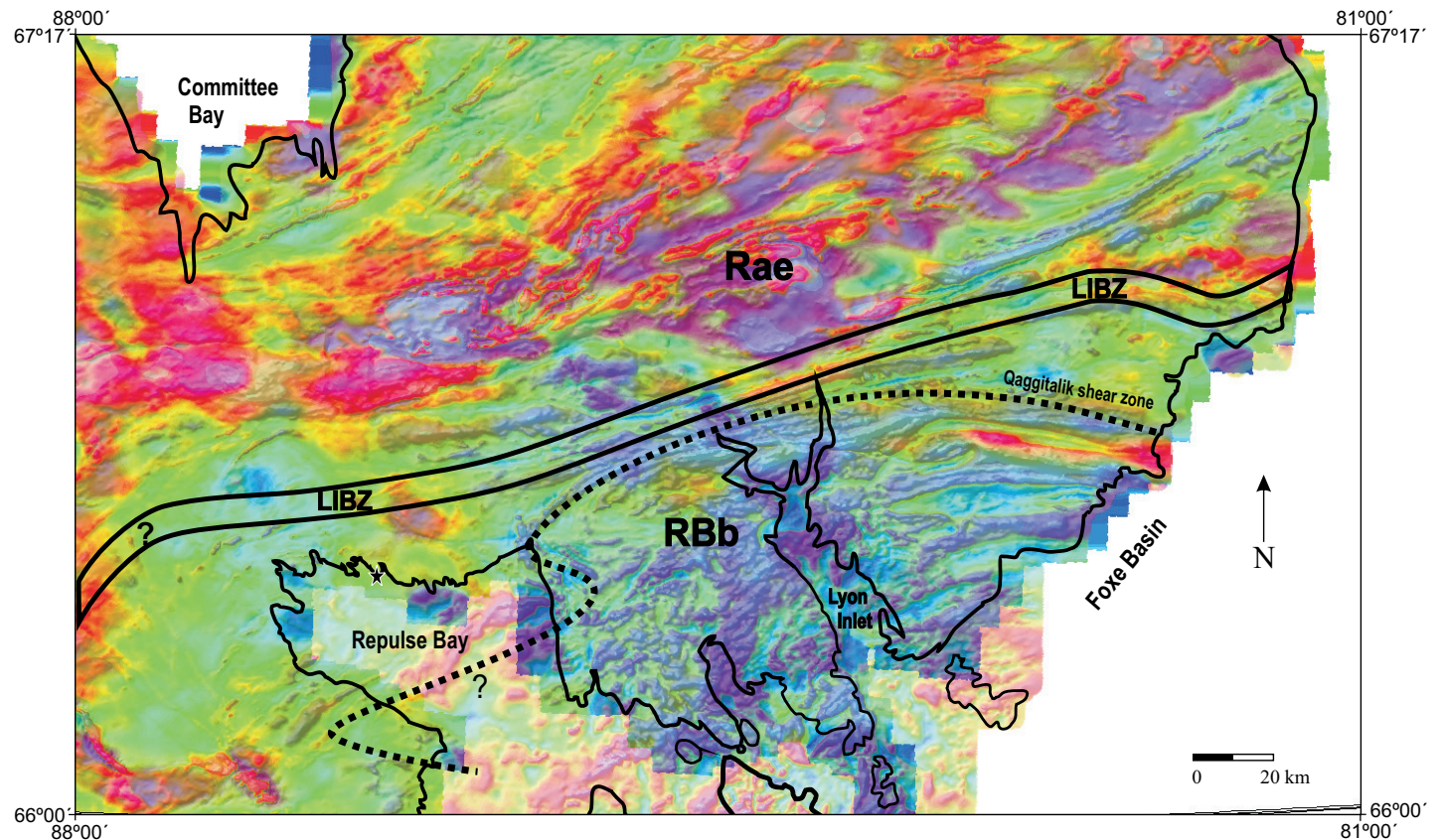
Figure 3. Combined airborne magnetic map and airborne radiometric map (equivalent U (eU); 800 m spacing) of the Repulse Bay block (RBb). Anomalous high magnetic properties in red and low in blue. High total U is in red, and low in blue. LIBZ – Lyon Inlet Boundary Zone.
