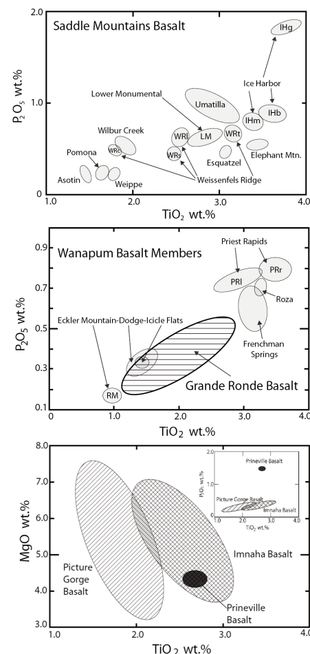
Figure 7. Variation diagrams showing compositions and differences of the seven Columbia River Basalt Group (CRBG) formations and selected members. Ranges of analyses are enclosed by lines. See Reidel et al. (2013a) and Reidel and Tolan (2013a) for a more complete listing of CRBG analyses.
