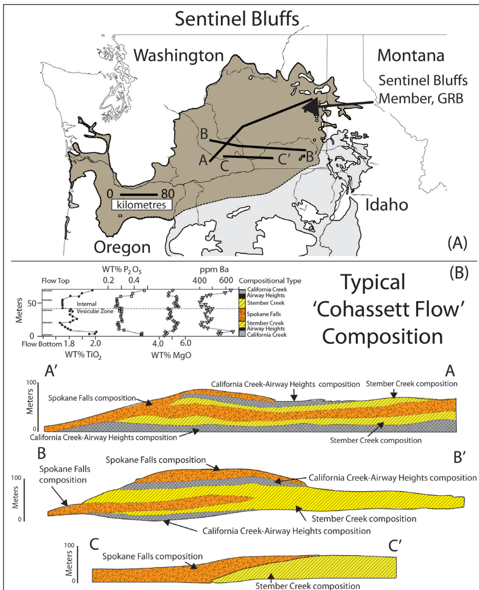
Figure 5. Extent of the Cohassett flow of the Sentinel Bluffs Member, Grande Ronde Basalt (GRB). Diagram shows the extent of the composite flow, compositions of the four individual flows that make up the composite flow (California Creek, Airway Heights, Stember Creek, and Spokane Falls), and cross sections through the flow that show the internal architecture of the composite flow. The cross sections are based on detailed analyses through the Cohassett flow along each section. See Reidel (2005) for details of the study.
