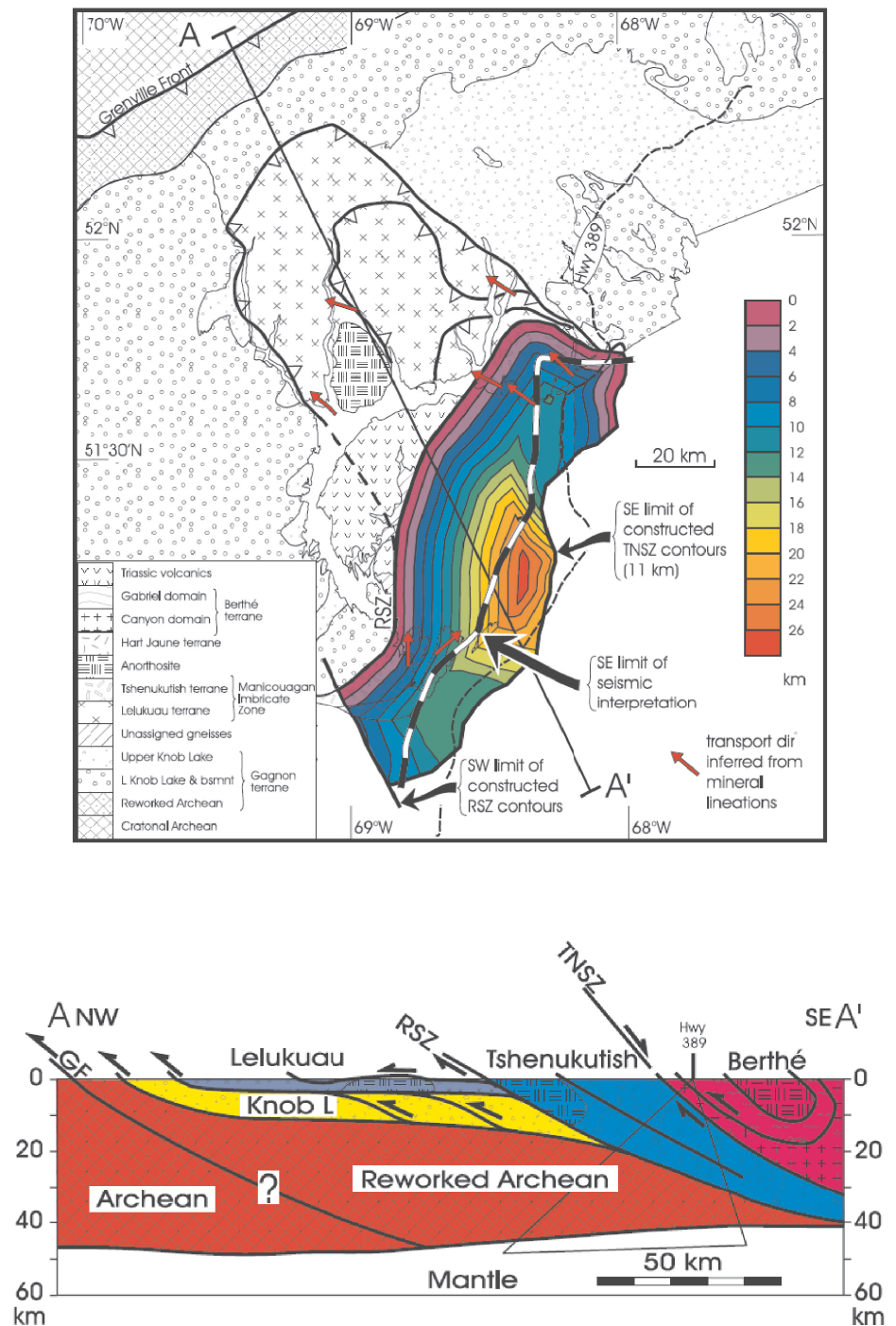
Figure 16. (a) Isopach map for the Tshenukutish terrane. Heavy dashed line is the southeastern limit of structure contours for which their position is constrained by observed reflectors. Red arrows show inferred transport directions for rocks within Tshenukutish terrane based on the predominant trends of mineral lineations. AA' is location of section below. (b) Vertical cross-section along line AA' (Figs. 15a, 16a). Depths of boundaries within the triangular field beneath the surface trace of Highway 389 are constrained by structure-contour maps derived from interpretation of Line 55. Outside that region, subsurface structure is based on extrapolation parallel to the regional tectonic trend of the Grenville orogen. Colour and ornament same as Figure 15a. From Hynes et al. (2000).
