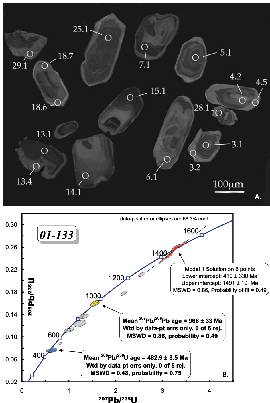
Figure 8. A: Cathodoluminescence image (CL) of zircon from sample 01-133. Note the narrow outer rims of relatively light-CL and without internal structure, that represent the Ordovician metamorphic overgrowth on the older ca. 1.0-1.5 Ga cores. B: Total concordia plot of zircon grains from 01-133. See text for further explanation, and Table 2 for the data.
