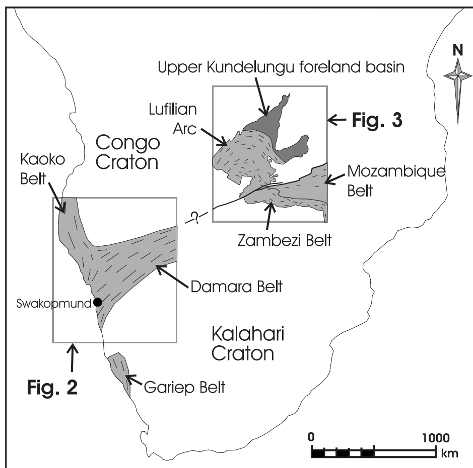
Figure 1. Relative locations of the Pan-African Damara Orogen and Lufilian Fold Belt in southern Africa (modified after Miller and Schalk 1980; Kampunzu and Cailteux 1999; Porada and Berhorst 2000).
