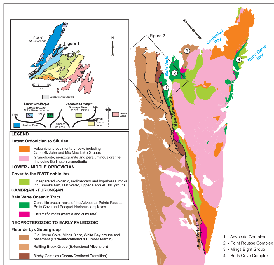
Figure 1. Simplified Geology of the Baie Verte Peninsula, northwestern Newfoundland (modified from Hibbard 1983 and Skulski et al. 2010). AAT: Annicop-squotch Accretionary Tract; BVBL: Baie Verte – Brompton Line; DBL: Dog Bay Line; DF: Dover Fault; GRUB: Gander River Untramafic Belt; HMT: Hungry Mountain Thrust; RIL: Red Indian Line.
