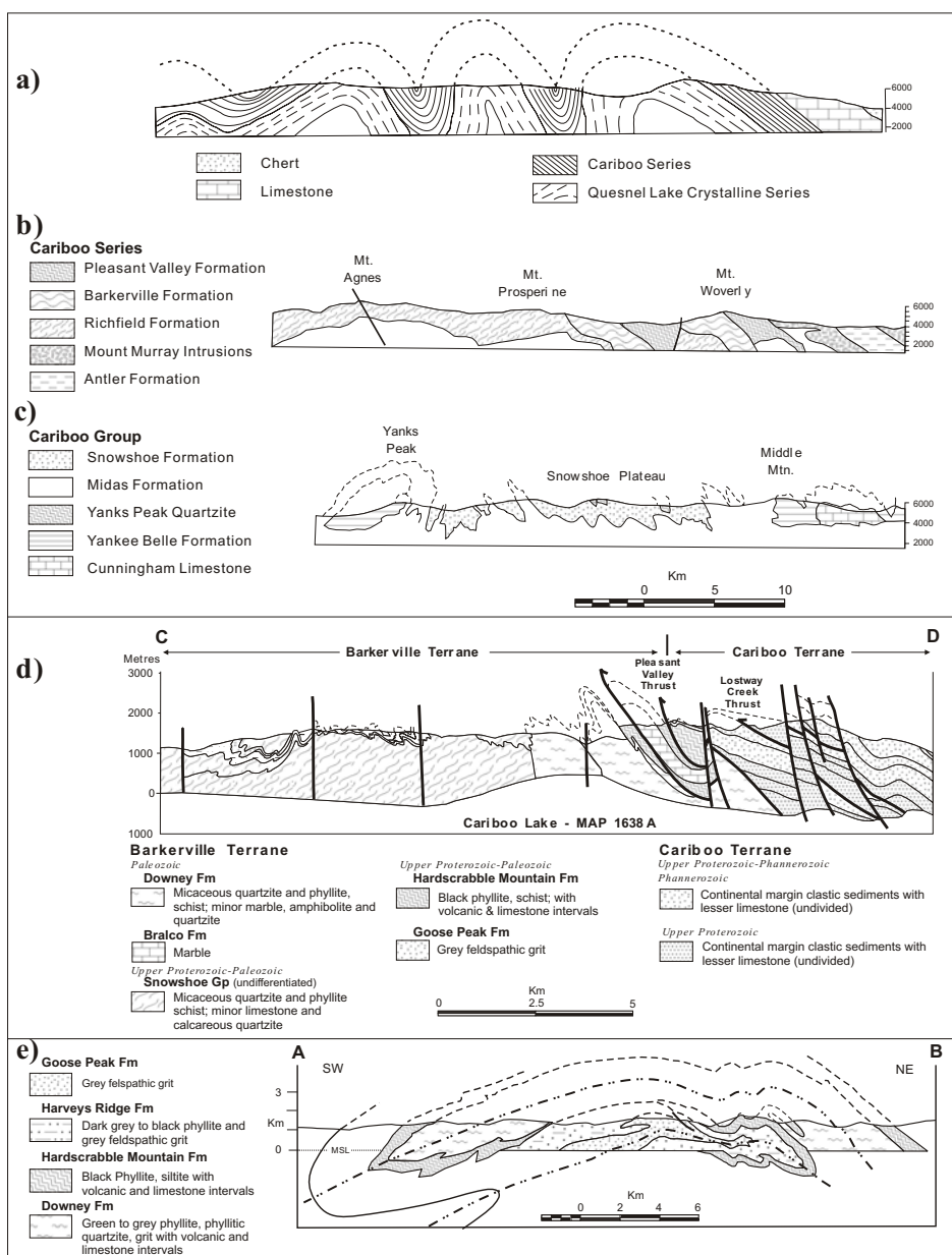
Figure 7. Evolution in interpretation of structural cross-sections for Cariboo Goldfield area. Section a) is after Bowman (1888), b) is after Johnston and Uglow (1926), c) is after Holland (1954), d) is after Struik (1988, and e) is after Schiarizza and Ferri (2003). The approximate locations of cross-sections d) and e) (C-D and A-B, respectively) are shown on Figure 5. Sections a), b) and c) are schematic only; because they are historical sections, they do not match the geology shown in Figure 5.
