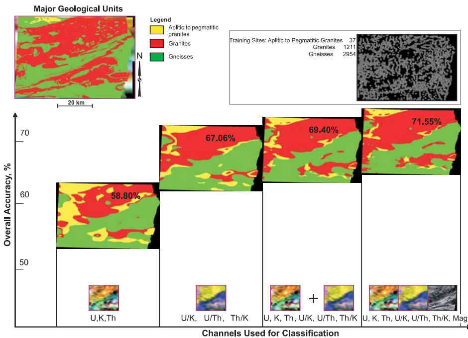
Figure 21. Supervised classification (prediction) of major tectonic divisions using a maximum likelihood algorithm applied to gamma-ray and magnetic data for the Melville Peninsula, Nunavut (see Figs. 6 and 7 for location). Training samples for each of the major tectonic units were gathered from legacy field data (point locations). Some of these were used for classification purposes whereas others were used for validation (cross-correlation) purposes. The accuracy, when compared to the check training sites, varied from close to 60% accuracy, when just using eTh, eU, and K for classification, to 72% when using both gamma-ray data (raw or elemental + ratios) and magnetic data.
