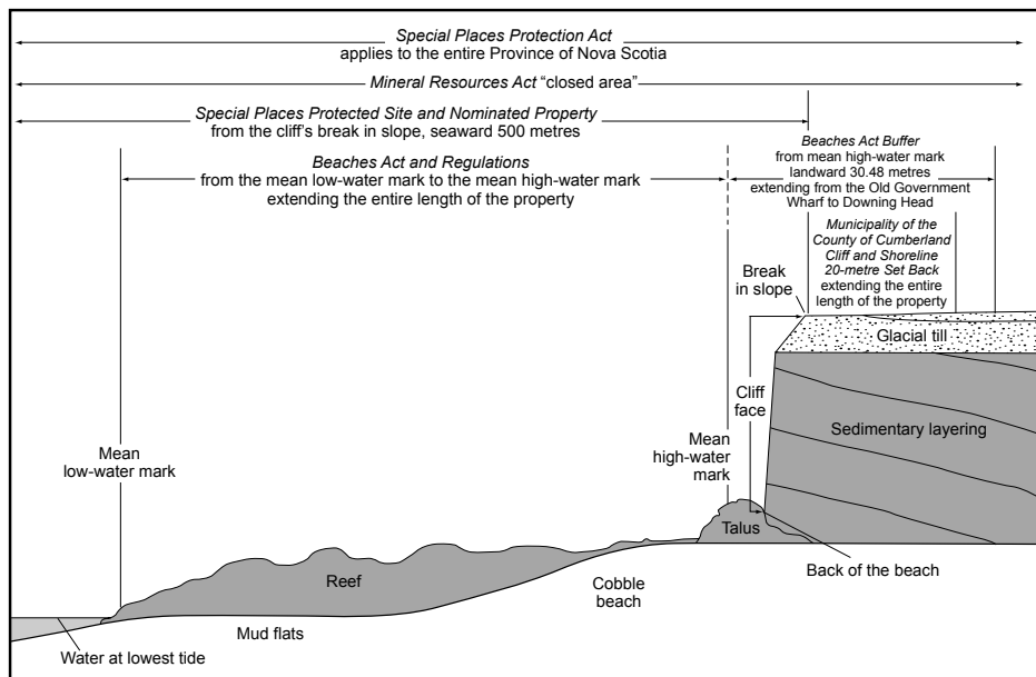
Figure 3. A diagram illustrating the Joggins Fossil Cliffs World Heritage Site, Nova Scotia, Canada, and the legislation that protects the site and its surroundings (after Joggins Fossil Institute 2007).
