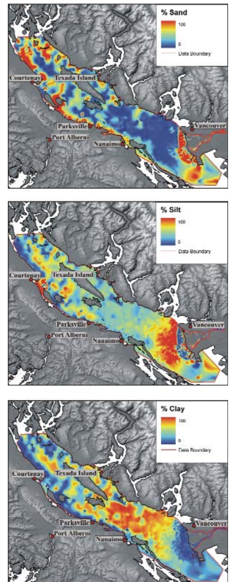
Figure 11. Surficial sediment distribution (% sand, silt and clay) on the seafloor of the Strait of Georgia, based on over 4,400 grab samples.
