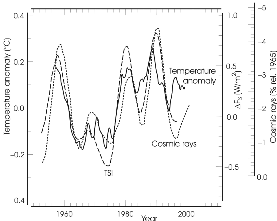
Figure 17. Annual variability in tropospheric temperature, TSI ( \Delta F_s ) and CRF. Note the reversed scale for CRF. Modified from Marsh and Svensmark (2003b) and Marsh et al. (2005).
