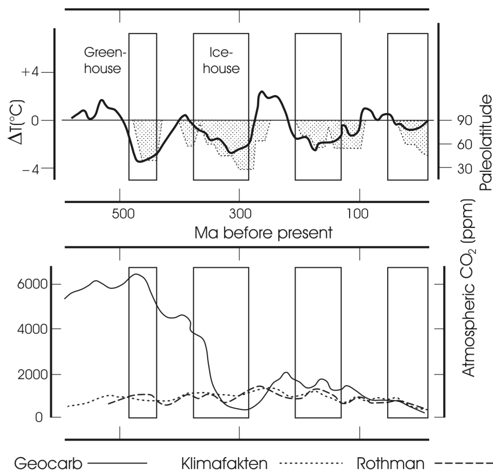
Figure 5. Phanerozoic climatic indicators and reconstructed p CO 2 levels. The curve in the upper set is the relative paleotemperature trend as calculated from the \delta^{18}\text{O} values of calcitic shells (Veizer et al., 2000). The dotted histograms mark the lowest paleolatitude (right-hand vertical axis) at which the ice rafted debris was observed in ancient sediments. The boxes represent cool climate modes (icehouses) and the intervening intervals the warm modes (greenhouses), as established from sedimentological criteria (Frakes et al., 1992). The bottom set of curves describes the reconstructed histories of the past p CO 2 variations (GEOCARB III) by Berner and Kothavala (2001), Klimafakten (Berner and Streif, 2000) and Rothman (2002). A recent argument by Royer et al. (2004) that the \delta^{18}\text{O} trend of Veizer et al. (2000) reflects the pH rather than the temperatures of ancient oceans is interesting, but this proposition, apart from being rather arbitrary, cannot explain the magnitude of the \delta^{18}\text{O} trend (Shaviv and Veizer, 2004a; Wallmann, 2004) and is also at odds with the paleoclimatological reconstructions (see Scotese, 2002; Boucot and Gray, 2001, and Boucot et al., 2004). As for the “critique” of Rahmstorf et al. (2004) see Shaviv and Veizer (2004b), http://www.phys.huji.ac.il/~shaviv/ClimateDebate , and de la Fuente Marcos and de la Fuente Marcos (2004).
