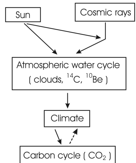
Figure 18. Schematic presentation of the sequence of events for a model based on celestial forcing as the principal climate driver. The dashed arrow is a feedback from the biosphere on climate, including its anthropogenic component.
