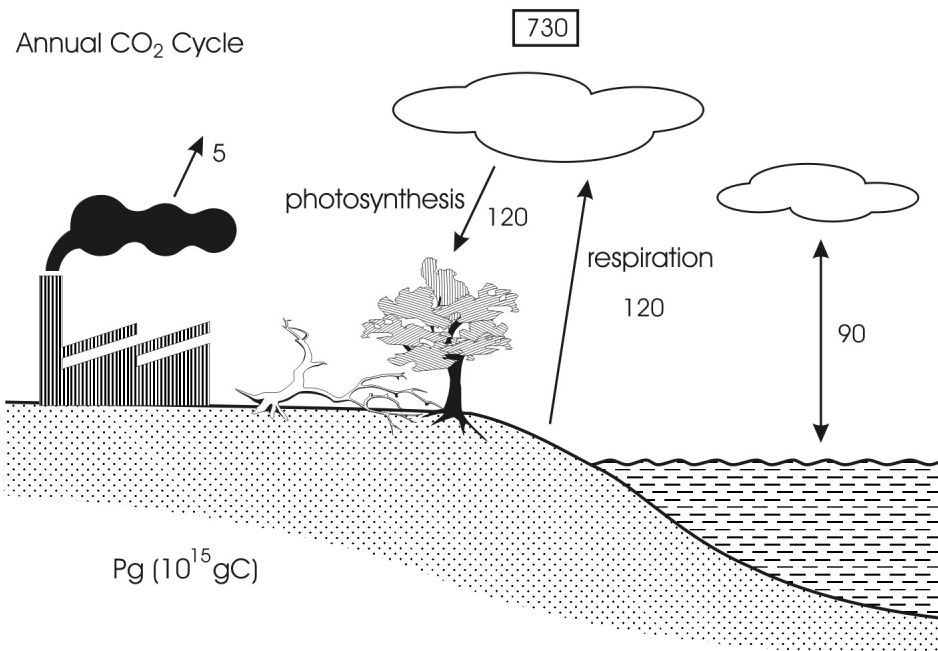
Figure 19. Simplified annual carbon cycle. Based on data in Prentice et al. (2001).
