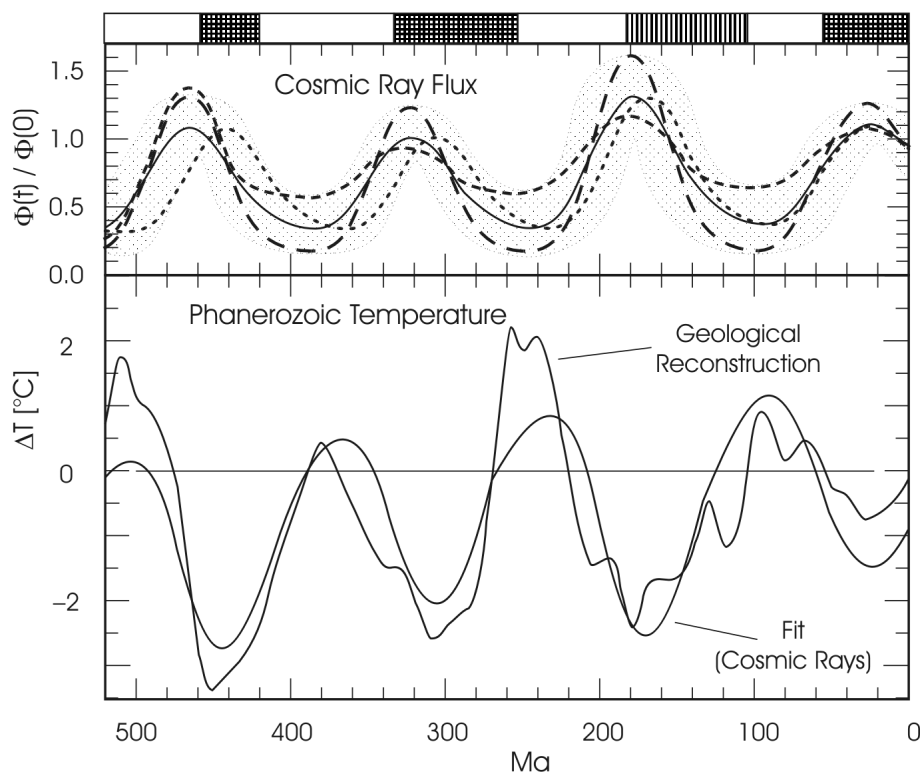
Figure 6. The variations in the cosmic ray flux ( \Phi ) and tropical seawater temperature variations ( \Delta T ) over the Phanerozoic. The upper curves describe the reconstructed trends for cosmic ray flux (CRF) within their uncertainty band (stippled). The bottom curves depict the smoothed temperature anomaly ("Geological Reconstruction") based on the \delta^{18}\text{O} record and the model cosmic ray flux ("Fit"). The peaks and valleys represent greenhouse and icehouse episodes as in Fig. 5. Note that no polar ice caps were as yet demonstrated for the third (hatched) icehouse. Adapted from Shaviv and Veizer (2003).
