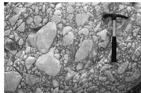
Figure 3 Facies problematica. Understanding of Earth's pre-Pleistocene glaciations is heavily reliant on the environmental interpretation of poorly sorted rocks called diamictites . Much past work, particularly in the Neoproterozoic, has simply assumed that such facies are tillites deposited directly under ancient glaciers. Such rocks however, form widely in non-glacial and glacial environments and are not uniquely diagnostic of episodes of cold climate. The environmental interpretation of such facies relies on examination of the overall depositional context (i.e., of the strata that lie above and below). As detailed sedimentological studies proceed, it is evident that many 'glacial' diamictites reported in the past are non-glacial mass-flow deposits preserved in marine successions and deposited under active tectonic conditions. True tillites appear to be rare in the Neoproterozoic: the record of ancient cold climates is dominantly preserved in offshore marine strata where primary glacial sediment was reworked by non-glacial process (e.g., Fig. 4). Unravelling climate from such non-fossiliferous strata is a challenge.
