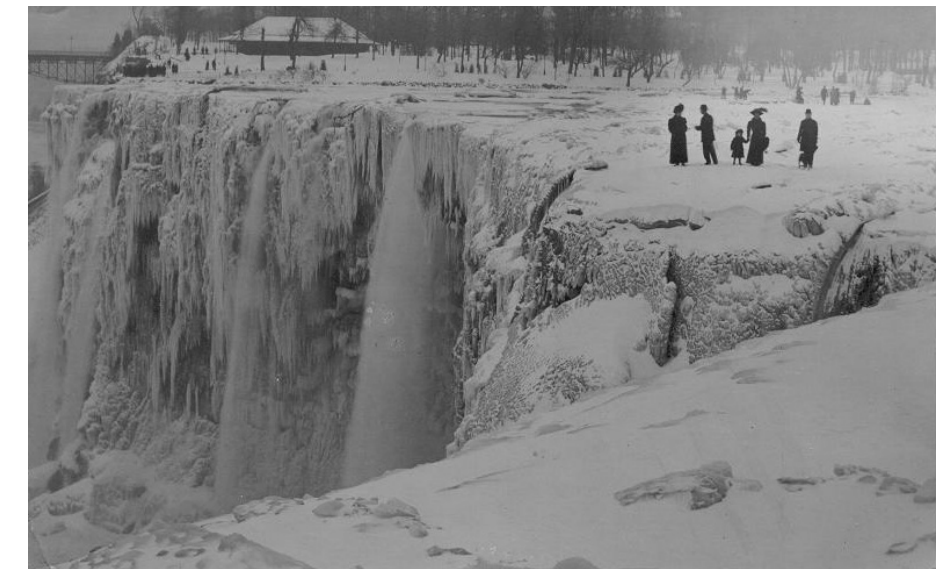
Figure 1 Frozen Earth: Niagara Falls in the winter of 1911. The possibility of a completely ice-bound planet has been a source of fascination for generations of scientists and society at large. Photograph courtesy of Steve Dibiase.
