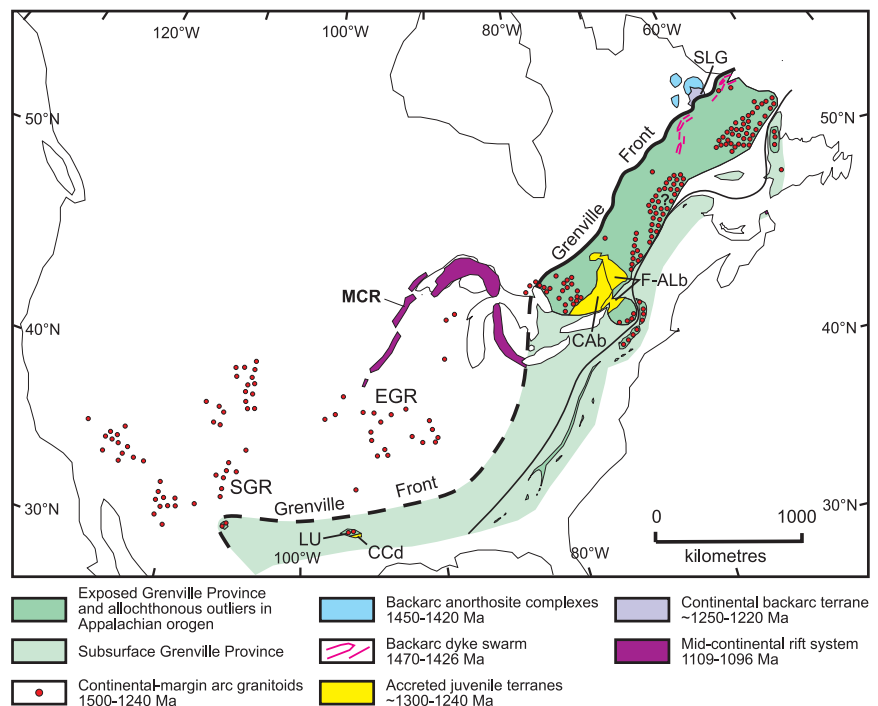
Figure 5 Sketch map of North America (modified from Rivers, 1997) showing the location of the Grenville Province and its extension to the southwest and outliers (LU - Llano Uplift). Mesoproterozoic arc rocks (red dots) occur within the Grenville Province and in the buried foreland (Southern and Eastern Granite-Rhyolite belts: SGR and EGR). Accreted late Mesoproterozoic terranes: Composite Arc belt (CAb), Frontenac-Adirondack Lowland belt (F-ALb), Coal Creek domain (CCd). Mesoproterozoic continental back-arc deposits include the Mid-continent rift (MCR), Seal Lake Group (SLG) (red beds and mafic sills), anorthosites and mafic dyke swarms.
