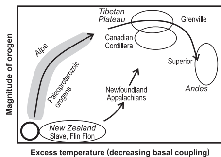
Figure 15 Orogenic pathways illustrated on a Hertzprung-Russell diagram, as modified by S. Ellis and C. Beaumont. Type orogens are shown for comparison to Archean, Proterozoic and Phanerozoic orogens of Canada.
