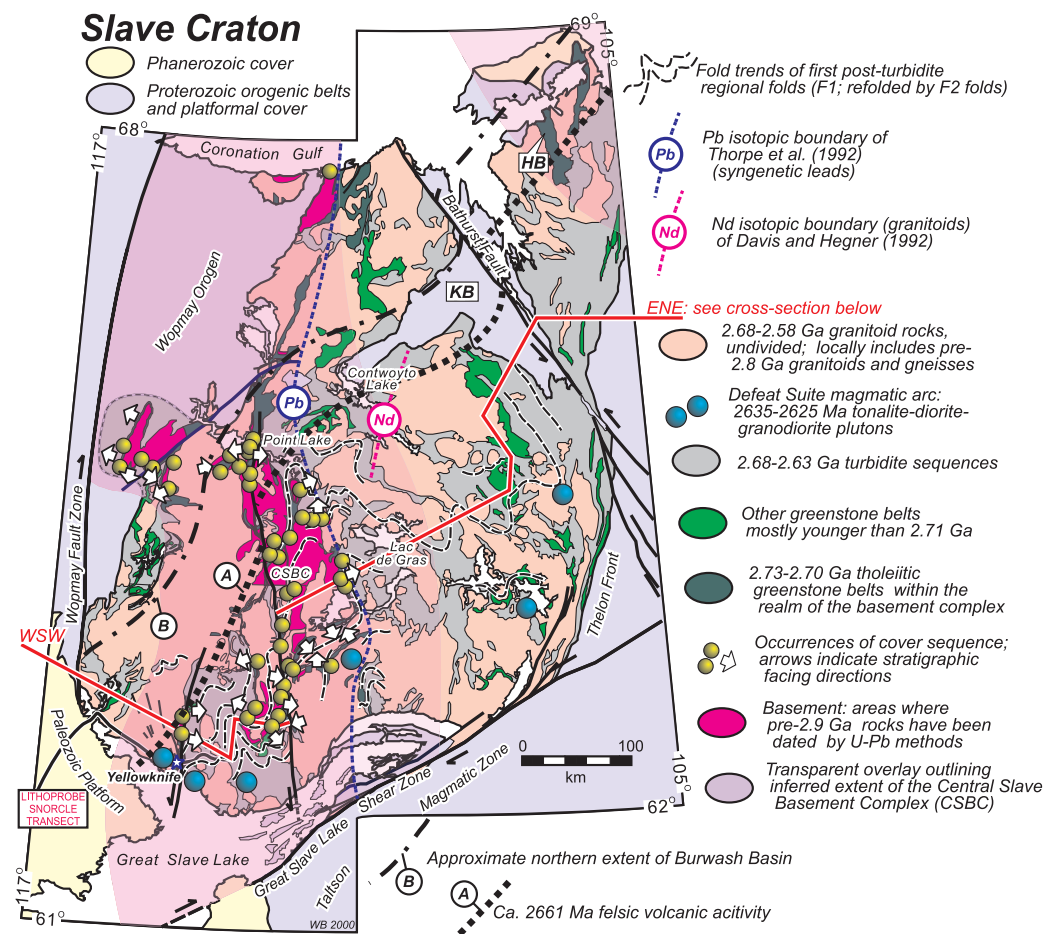
Figure 12 Geological map of the Slave craton. Transparent overlay (light purple) outlines probable, and possible (Hope Bay block), distribution of ancient basement. Line “A” outlines an arc of 2661 Ma felsic volcanic centres; line “B” outlines an approximate northwestern boundary to the “Burwash Basin”; all post-Burwash volcanic and turbiditic rocks occur to the northwest of the line.
