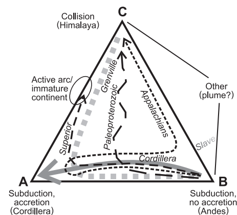
Figure 14 Orogenic classification diagram developed at the workshop to describe the development of orogens in terms of subduction, accretion and collision. Additional end-members may be necessary in some orogens to describe non-plate tectonic processes.
