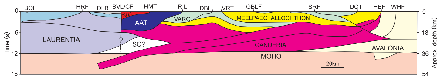
Figure 4 Interpreted seismic reflection profile of Meelpaeg transect (from van der Velden et al., in press). Migrated reflection data is plotted at 1:1 assuming a velocity of 6000 m/s. Colour scheme is similar to that of Figure 3. The Meelpaeg allochthon is bounded at its hanging wall by a low-angle normal fault (GBLF). BOI: Bay of Island ophiolite; HRF: Humber River fault; BVL: Baie Verte Line; CF: Cabot fault; NDA: Notre Dame arc; HMT: Hungry Mountain thrust; AAT: Annieopsquotch accretionary tract; SC: subduction complex of underplated material; VARC: Victoria arc; RIL: Red Indian Line; DBL: Dog Bay Line; DLB: Deer Lake basin; VRT: Victoria River thrust; GBLF: Great Burnt Lake fault; SRF: Salmon River fault; DCT: Day Cove thrust; HBF: Hermitage Bay fault; WHF: White Horse fault.
