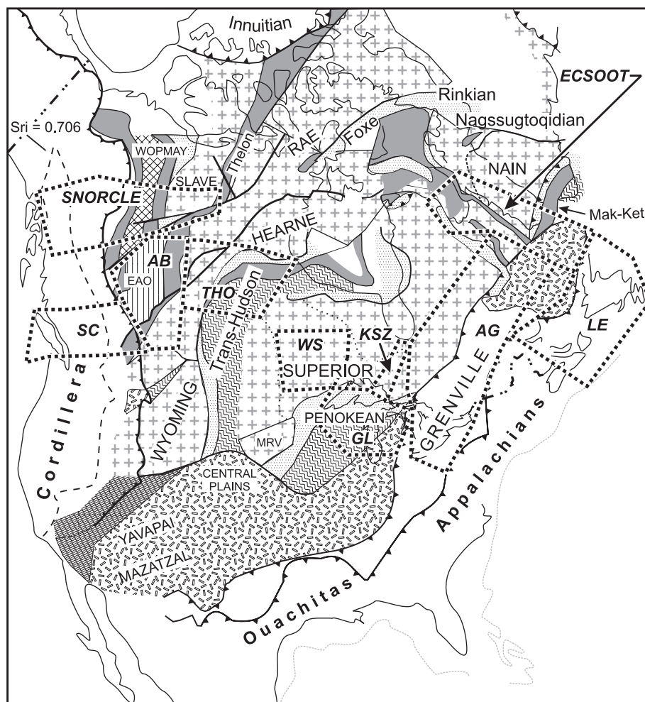
Figure 1 Precambrian tectonic domains for North America classified using U-Pb ages and Nd signature. The Sri (initial 87\text{Sr}/86\text{Sr} ) line in the Cordillera marks the western edge of thick Precambrian crust (from Armstrong, 1988). EAO: East Alberta orogen; MRV: Minnesota River valley gneiss; Mak-Ket: Makkovik-Ketilidean. Modified from Hoffman (1989). Detailed legend for Paleoproterozoic units is given in Figure 8; cross pattern indicates Archean crust. LITHOPROBE transects: AB: Alberta basement; AG: Abitibi-Grenville; ECSOOT: Eastern Canadian Shield onshore-offshore transect; KSZ: Kapuskasing structural zone; LE: Lithoprobe east; SNORCLE: Slave-Northern Cordillera Lithospheric evolution; SC: Southern Cordillera; WS: Western Superior; THO: Trans-Hudson orogen.
