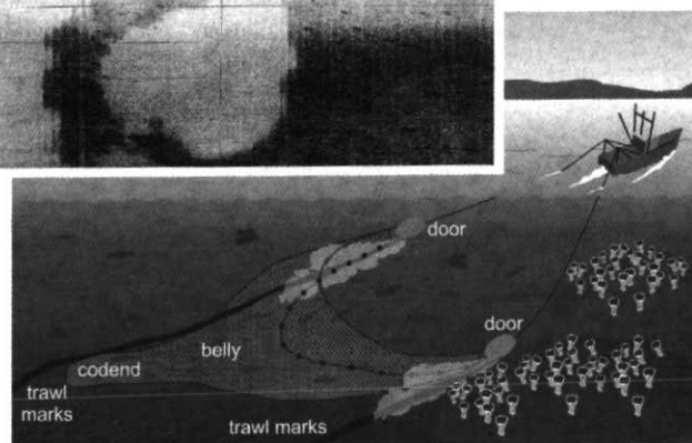
Figure 7 Sidescan sonar showing paired trawl marks on seafloor crossing sponge bioherms. These marks are created when net doors, weighing up to 2 tonnes, are dragged across the seafloor. Lower right sketch after Christen, 1999.
