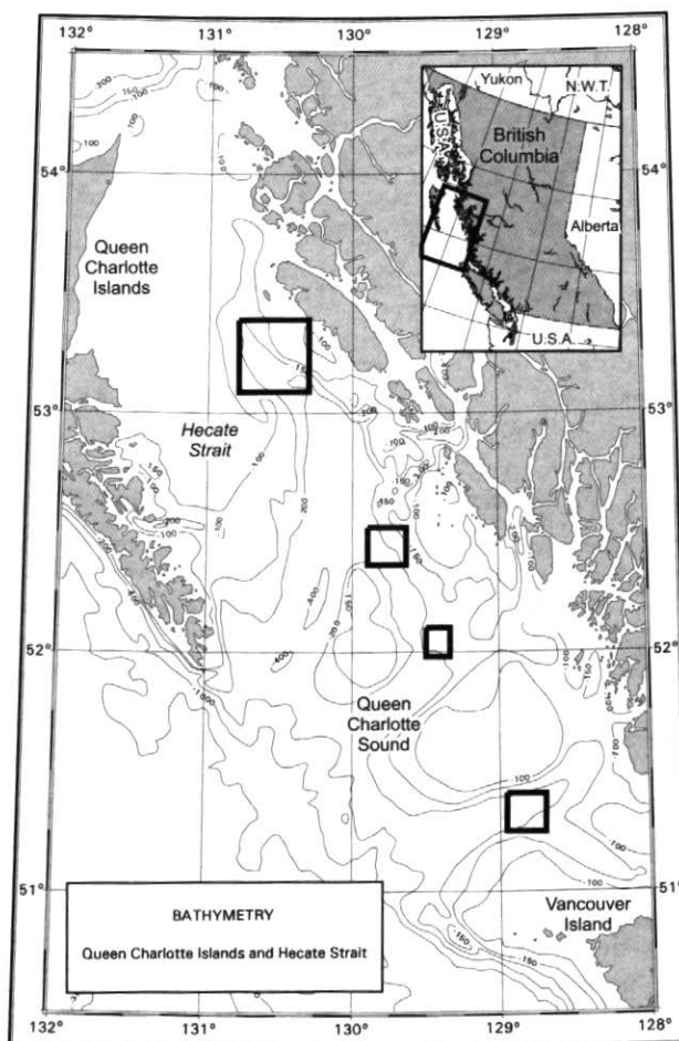
Figure 1 Bathymetry of the western Canadian shelf. Sponge reef areas surveyed during cruise PGC9901 are indicated within black rectangles. Depth contours in metres.
