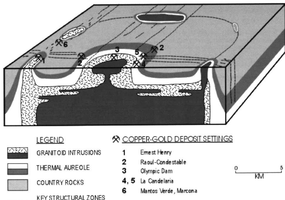
Figure 1 Cartoon placing a number of the world's best-known iron oxide copper-gold deposits in position relative to magmatic bodies, shown here as granitoid intrusions. Note that deposits range from close to distant with respect to a controlling magma body. After Wall, 2000.
