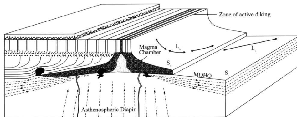
Figure 11 The "tent-shaped" model of Nicolas et al. (1988) based on structural evidence from the Oman ophiolite.
