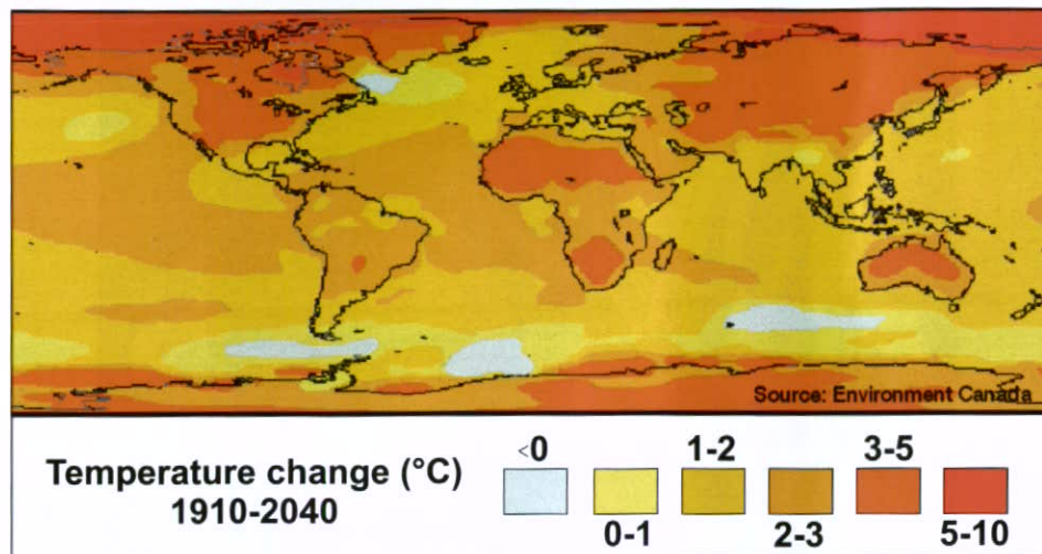
Figure 2 Map showing predicted differences in global surface air temperatures between 1910 and 2040, based on a global climate model. The greatest differences are predicted to be at high latitudes and in the interior of continents (Environment Canada, 1993).
