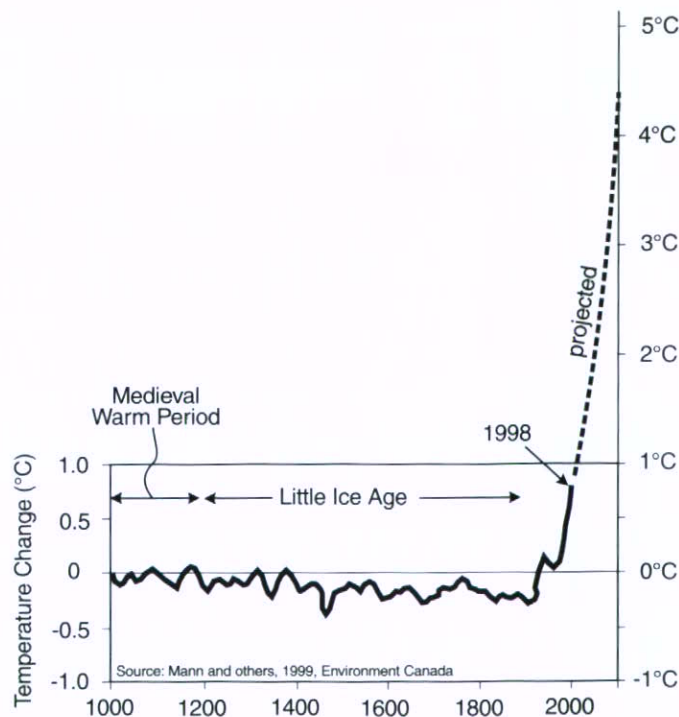
Figure 3 Average northern hemisphere temperatures during the last millennium and projected temperature rise over the next 100 years (adapted from Mann et al. , 1999).
