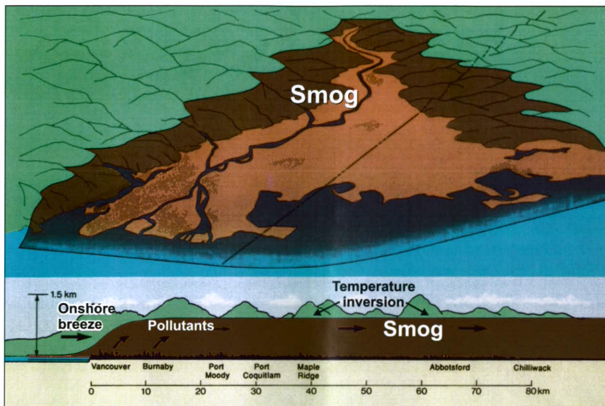
Figure 6 Pollutants can be trapped beneath a layer of warmer air in the Fraser Valley east of Vancouver. Airborne pollutants are typically carried east from Vancouver by prevailing westerly winds (Turner and Clague, 1999).
