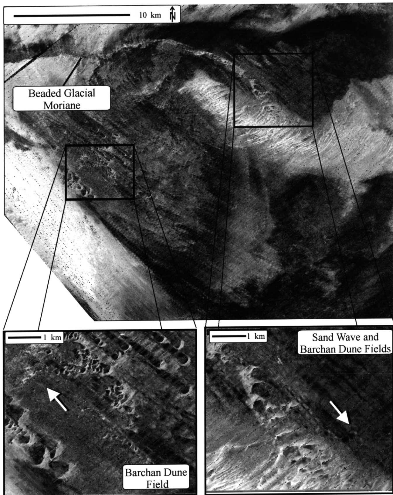
Figure 9 Backscatter mosaic on a section of Browns Bank is plotted with low-amplitude backscatter shown as lighter tones. The barchan dunes and sand wave field show up as zones of low backscatter. Less obvious on the shaded relief image (Fig. 8), the backscatter mosaic suggests a more subtle drape of low backscatter material, likely caused by thin layers of sand overlying a gravel lag, distributed in wispy and patchy patterns aligned in a general clockwise gyre pattern. The seabed found between the horns of the barchan dunes shows a relatively higher backscatter signature, attributable to turbulent scouring of the seabed as currents flow over the bedform, exposing a gravel lag.
