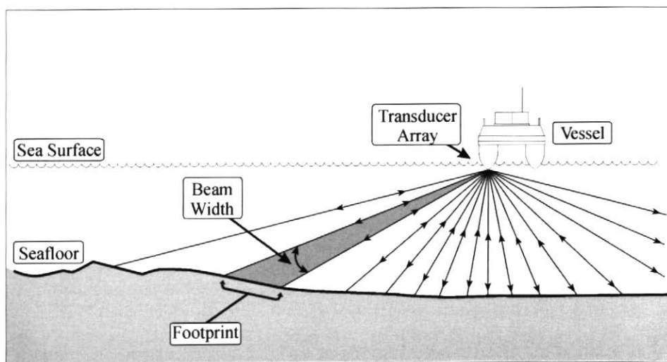
Figure 1 A hull-mounted multibeam system measures a sequence of depths across a fan-shaped arc sweeping to both port and starboard beneath the survey vessel. The arc is divided into a number of distinct and separate beams, which impinge the seabed over an area, or footprint, that expands with the distance between the transducer and the seabed.
