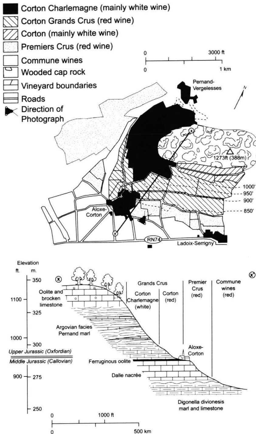
Figure 1 Plan and cross-section of the Hill of Corton, Côte d'Or wine-producing region of France, (a butte) showing the relationship of the geology to vineyard designations as Corton Charlemagne Grand Cru, Corton Grand Cru, Corton (white and red), Premier Cru (red), and Commune wines. Based on Figure 4.15 of Wilson (1998) with modification and additions of vineyard boundaries and designations from Comité Interprofessionnel des Vins de Bourgogne (undated).
