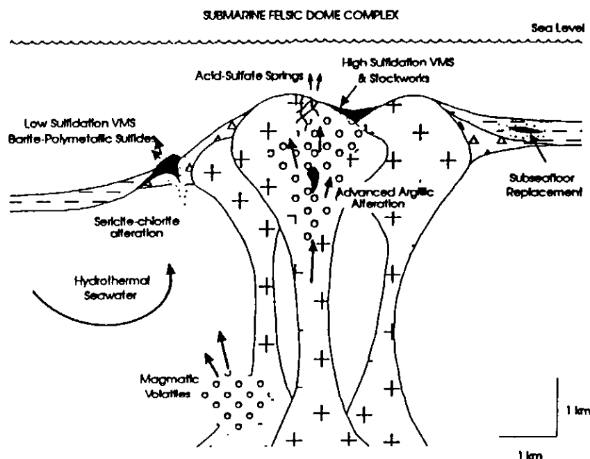
Figure 5 Schematic section of a high-sulphidation VMS environment in relation to a felsic dome complex, from John Thompson's presentation. Now published in Sillitoe, R.H., Hannington, M.D. and Thompson, J.F.H., Economic Geology , 1996, v. 91, p. 204-212.
