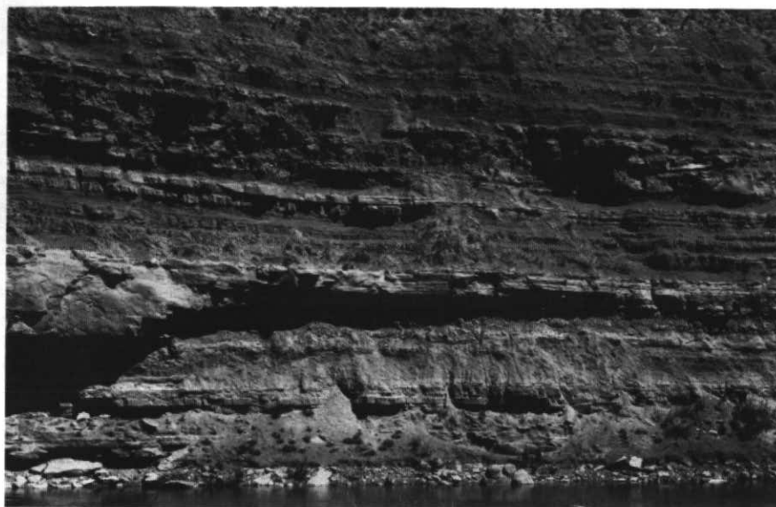
Figure 3 A typical channel sandstone lens within the St. Mary River Formation of southwestern Alberta. Note the lack of deformation of the sandstones on the margins of the lens and the horizontal nature of beds surrounding the sandstone lens even though maximum burial depth has exceeded 2000 m. This geometry is only possible if there is no significant differential compaction between the floodplain mudstones and sandstones.
