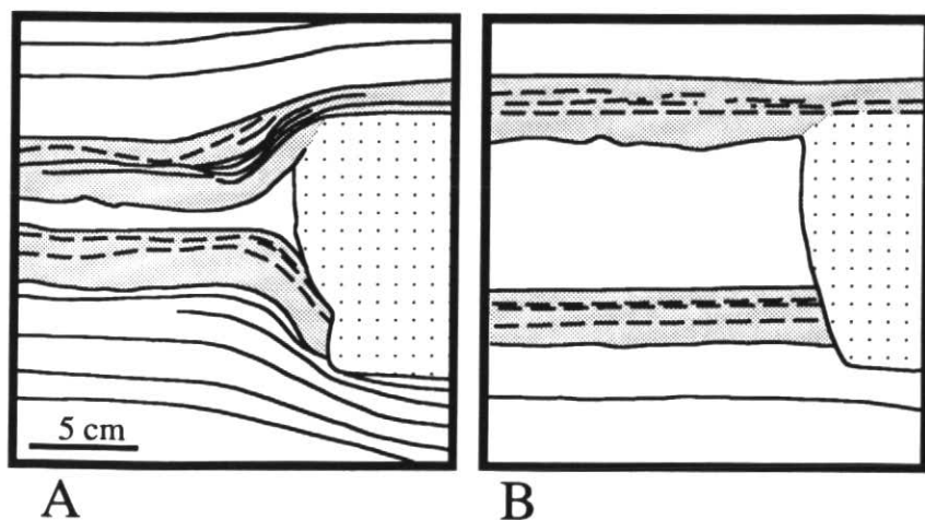
Figure 4 The lateral facies relationships at the margin of a sandstone lens and adjacent mudstones in a marine deposit. (A) illustrates the effects of large differences in initial sediment porosity between sands and muds on differential compaction, and (B) shows the original depositional configuration after decompaction. After Baldwin (1971).
