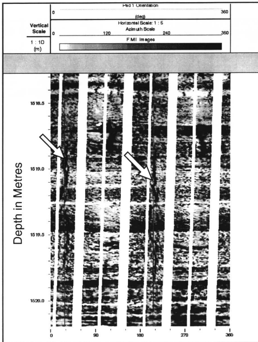
Figure 20 A Formation Micro-imager record from a western Canadian well that shows a semi-vertical drilling-induced fracture intersecting the borehole at N35°E and S215°W (arrows). This orientation coincides closely with S_{Hmax} determined from breakouts in nearby wells.
