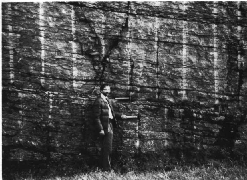
Figure 11 Offset boreholes exposed along the St. Laurent exit ramp off Autoroute 50 in Hull, Quebec. The average direction of offset is 070^\circ , which coincides well with regional S_{Hmax} orientations determined from hydraulic fractures, breakouts and earthquake focal mechanisms. Details are given by Wallach et al. (1995).
