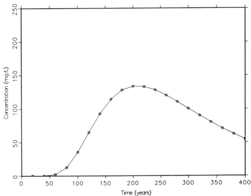
Figure 4 Chloride concentration in aquifer for clay liner.
