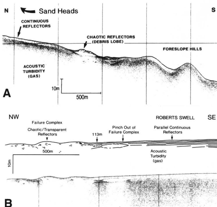
Figure 6 (A) Huntce seismic profile from near base of delta slope seaward of Sand Heads. Parallel continuous reflectors with acoustic turbidity (fog-like seismic character which masks structure deeper than a few metres), characteristic of gassy, undisturbed muds and mounded chaotic reflectors of debris flow lobe. For location, see Figure 1. (B) Huntce profile, with interpretation from base of delta slope near Roberts Bank. Chaotic and transparent reflectors which attenuate seismic signal represent sandy failure deposits, and interfinger with gassy, undisturbed muds.
