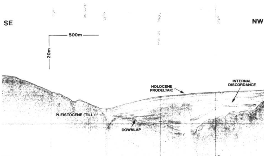
Figure 3 (A) Side-scan sonar image (Klein 100 kHz) and (B) corresponding high-resolution seismic profile (Huntec Deep Tow) showing Pleistocene deposits overlain by Holocene prodeltaic sediments. Using only the sonograph, it would be difficult to determine whether the dark patches represented a surficial deposit of dense material (e.g., Fig. 13) or an outcrop exposure of an underlying unit. Note fine-scale stratigraphic detail visible on seismic profile. For location, see Figure 1.
