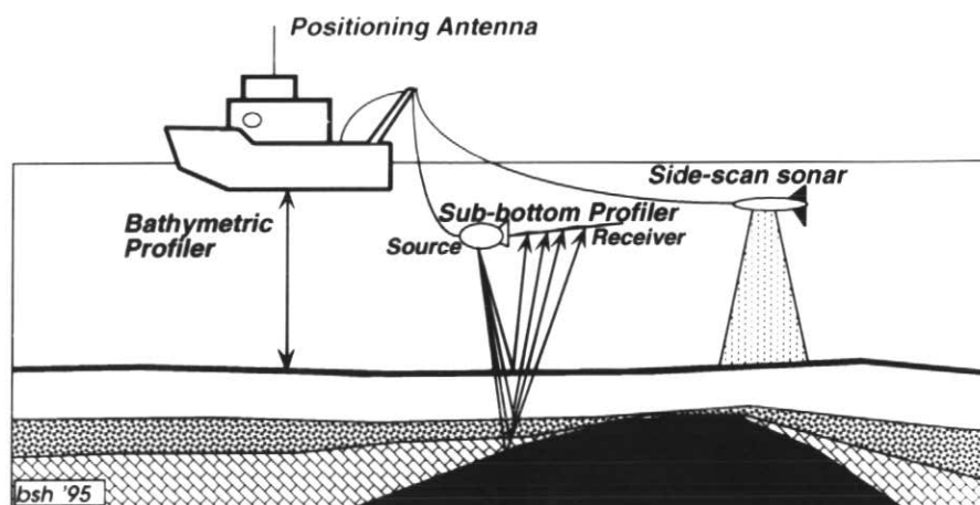
Figure 2 Illustration of simultaneous collection of bathymetry (hull-mounted system), sub-bottom profiler (high-resolution seismic) and side-scan sonar data during marine geophysical survey. Ship's position fixed using satellite-based system such as GPS. Location of profiler and side-scan towfish with respect to antenna (setback) determined by acoustic positioning systems mounted to towfish (for detailed work) or (for reconnaissance work) using cable length out, visual estimate (surface tow systems) or post-survey calibration to bathymetry data.
