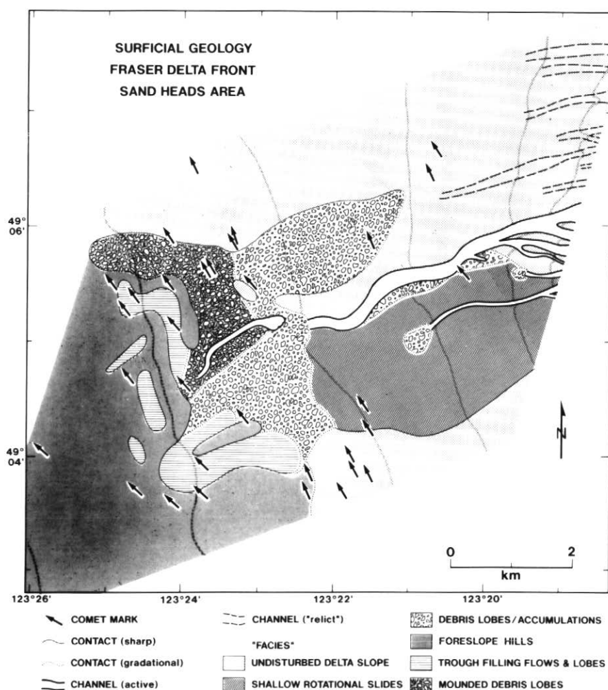
Figure 8 Surficial geologic map of the sea floor seaward of the mouth of the Main Arm of the Fraser River (see Fig. 1), prepared using side-scan sonographs, high-resolution seismic profiles, bathymetry and cores. Rapid sediment deposition on relatively steep slopes has led to the development of various failure-related morphological elements. Comet marks are current-formed scour marks around sea-floor debris, and can be used to identify dominant current direction. These are equivalent to the obstacle-induced sediment drifts of Fader and Buckley (in press).
