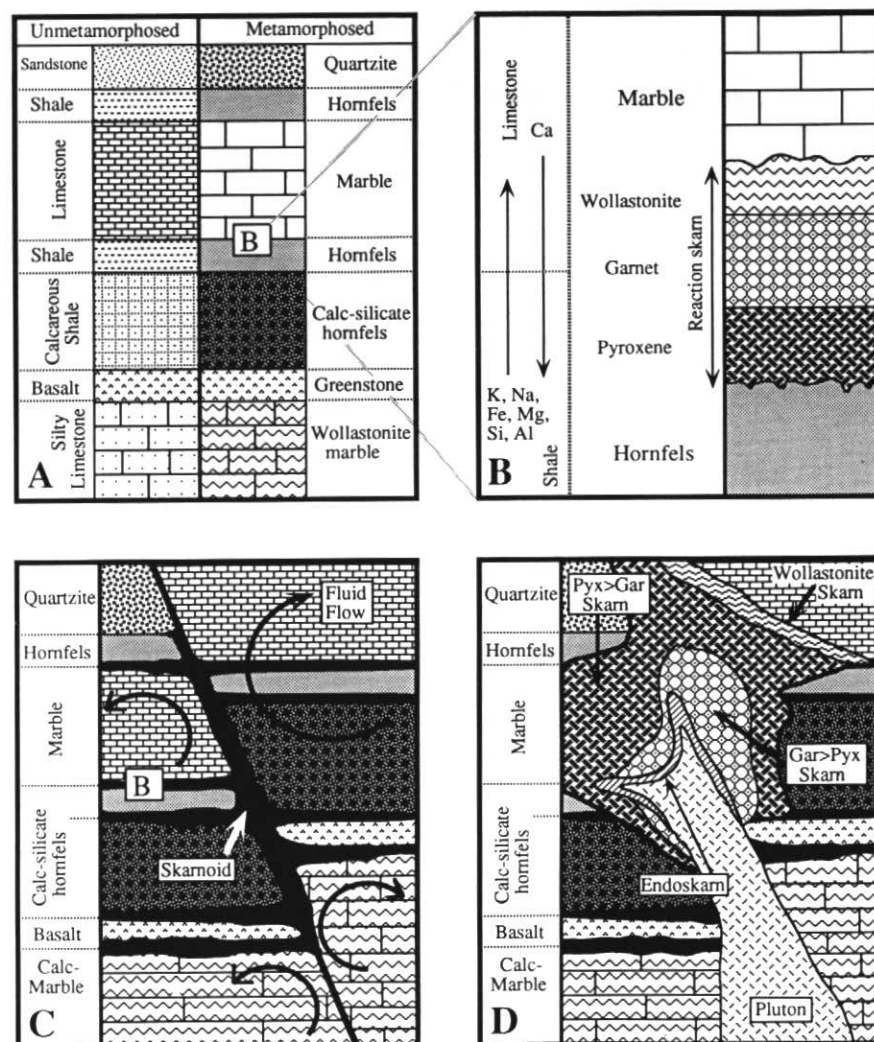
Figure 1 Types of skarn formation: (A) Isochemical metamorphism involves recrystallization and changes in mineral stability without significant mass transfer; (B) Reaction skarn results from metamorphism of interlayered lithologies, such as shale and limestone, with mass transfer between layers on a small scale (bimetasomatism); (C) Skarnoid results from metamorphism of impure lithologies with some mass transfer by small-scale fluid movement; (D) Fluid-controlled metasomatic skarn typically is coarse grained and does not closely reflect the composition or texture of the protolith.
