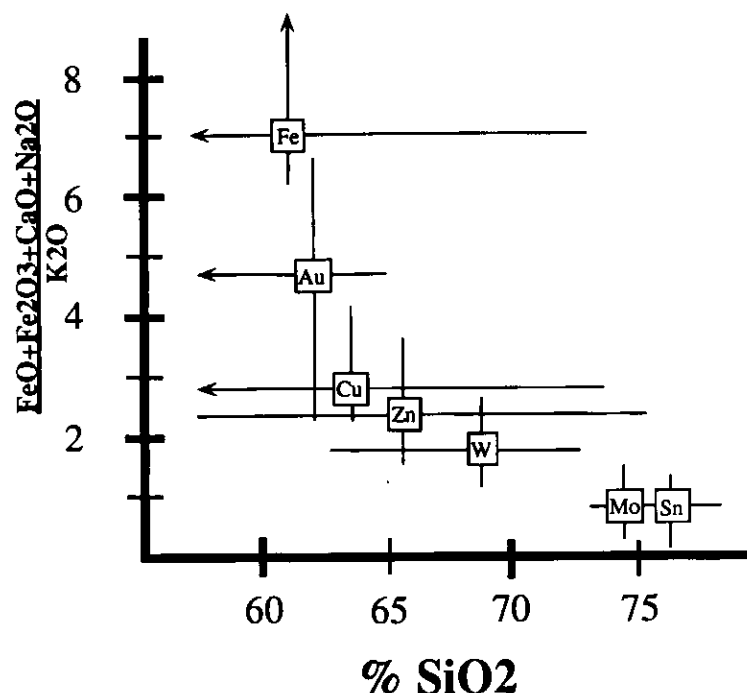
Figure 5 Average composition of plutons associated with different skarn types. Modified from Meinert et al. (1990).
