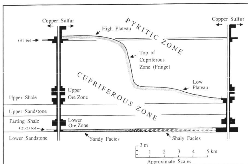
Figure 5 Schematic diagram showing the inverse correlation between the thickness of the cupriferous zone and the amount of mineralization in the combined No. 21 and No. 23 beds at White Pine, Michigan. Vertical exaggeration approximately 300×. See text for interpretation. From Brown (1970).
