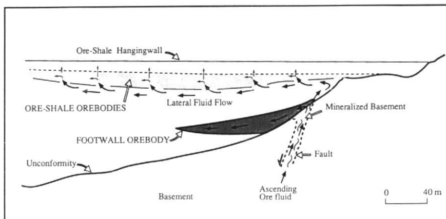
Figure 9 Interpretative diagram depicting the mineralization process for Footwall and Ore-shale orebodies in the Zambian copperbelt. Modified after Annels (1989).
