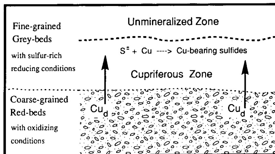
Figure 2 General deposit-scale model for sediment-hosted stratiform copper deposits. The heavy dotted line indicates the furthest advance of copper into the basal grey bed unit.
