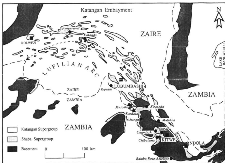
Figure 7 Location of major ore deposits in the Lufilian Arc of Zaire and the continuation of this copperbelt into Zambia. For location, see Figure 1.
