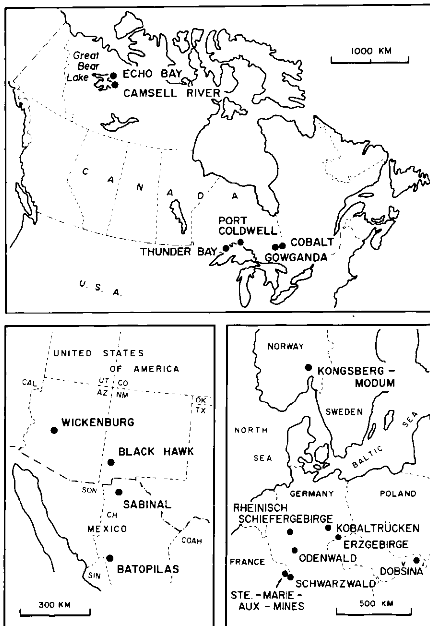
Figure 1 Location map for five-element vein deposits in Canada, the United States, Mexico and northern Europe. Four general localities — Rheinisch Schiefergebirge, Odenwald, Schwarzwald and Erzgebirge — are regions in Germany containing more than one deposit. The point for Kobaltrücken illustrates the general location of these veins in Thuringa and the Harz Mountains.
