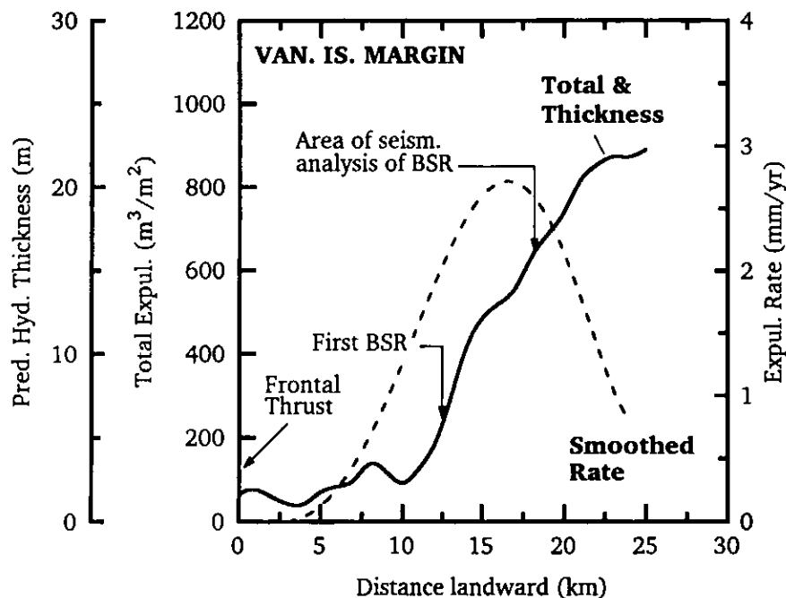
Figure 9 The estimated total amount of fluid ( m^3 ) expelled through an area of the sea floor ( m^2 ) as that area moves landward and is incorporated in an accretionary wedge. The model thickness of hydrate as a function of distance landward from the deformation front, estimated as described in the text, is also shown.
