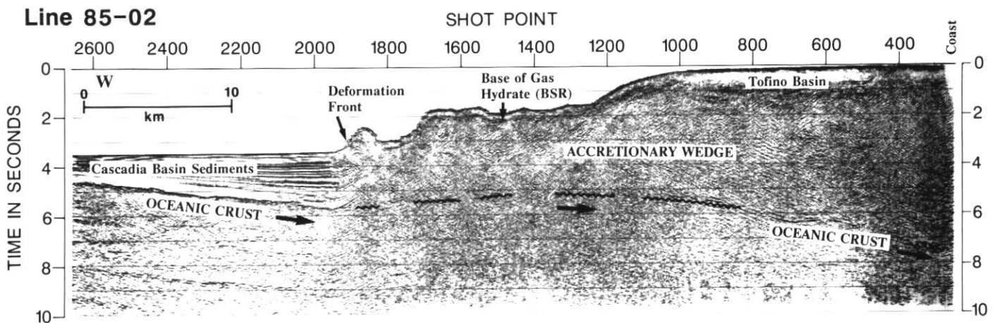
Figure 3 A multi-channel seismic section across the margin of Vancouver Island from the deep-sea basin to the coast, illustrating the position of the hydrate BSR. The incoming sediments of Cascadia Basin are about 2.5 km thick at the deformation front. The location of the section is shown in Figure 4.
