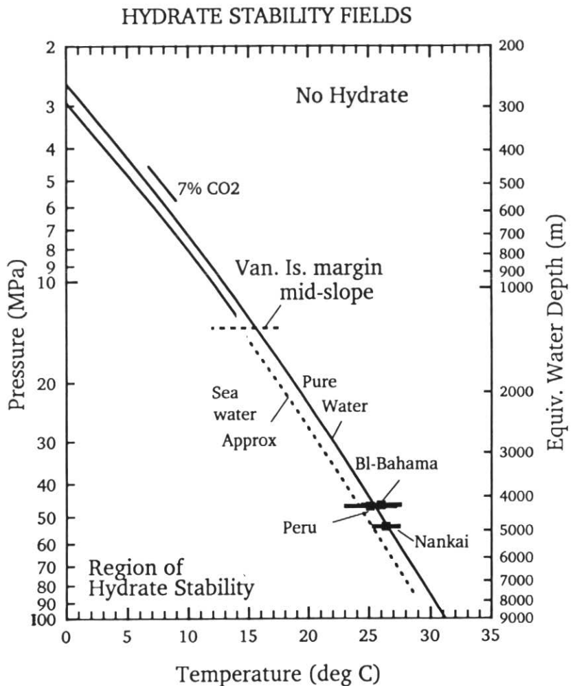
Figure 2 The stability field for methane hydrate in pure water. The influence of a small amount of CO 2 and of seawater salinity are illustrated. In situ calibrations of the hydrate BSR are shown along with the pressure (water depth) for the mid-slope study area off Vancouver Island.
