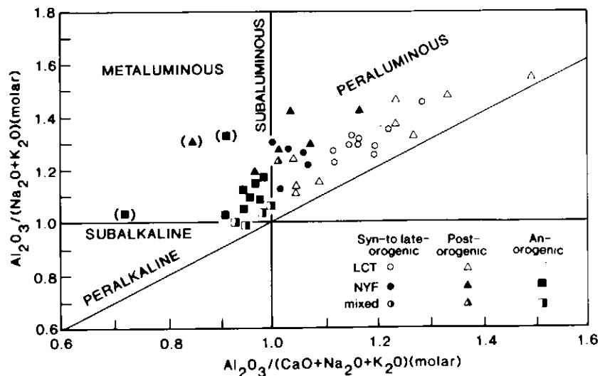
Figure 12 Fertile granites in the alumina saturation (Shand index) diagram (modified after Maniar and Piccoli, 1980, from Černý, 1991a), coded by tectonic affiliation and geochemical signature.
