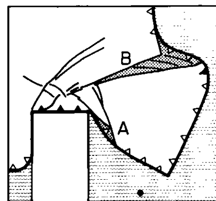
Figure 2 Extensional basins (A and B) formed during asymmetric lateral extrusion, based on plasticine experiment from Peltzer and Tapponnier (1988). Dot indicates finite rotation pole.
