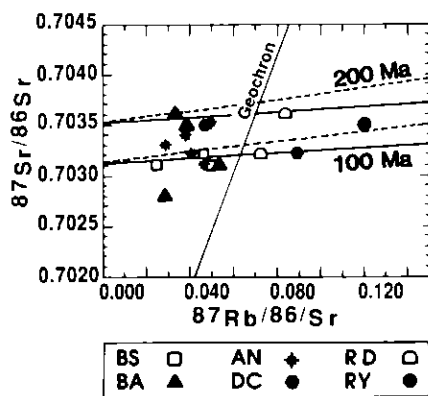
Figure 4 Rb-Sr systematics of Mount Garibaldi and Garibaldi Lake basalts (BS), basaltic andesites (BA), andesites (AN), dacites (DC), rhyodacites (RD), and rhyolites (RY). Note that the basalts, basaltic andesites, and andesites lie to the left, whereas more siliceous lavas generally plot to the right of the Geochron (4600 Ma isochron through BABI [Basaltic Achondrite Best Initial]). The Mount Garibaldi and Garibaldi Lake rocks define an array between 100 Ma (solid) and 200 Ma (dashed) reference isochrons which are compatible with K-Ar, Rb-Sr and U-Pb dates for basement Coast Plutonic Complex rocks (Mathews, 1972; Woodsworth, 1977; Armstrong, 1988).
