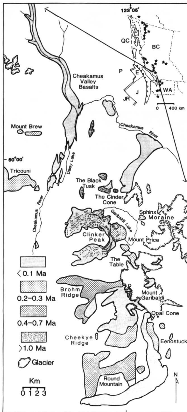
Figure 1 Timing and distribution of Pleistocene-Holocene volcanic rocks in the dominantly dacitic Mount Garibaldi and andesitic Garibaldi Lake volcanic fields. Inset illustrates the configuration of the Juan de Fuca ridge system (JR), Queen Charlotte fault system (QC), and Juan de Fuca (J), Explorer (E), and Pacific (P) plates along the continental margin of British Columbia (BC) and Washington (WA). Stars show Quaternary volcanic centres.
