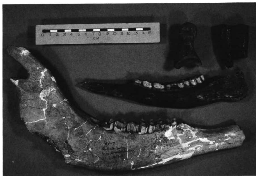
Figure 1 Quaternary fossils from the South Saskatchewan River Valley, Alberta and Saskatchewan. Top left: extinct camel ( Camelops hesternus ) lower molar, Kansan age, Island Bluff, Medicine Hat; top right: giant sloth ( Nothrotheriops shastense ) toe bone (proximal phalanx), Kansan age, Low Bluff, Medicine Hat; centre: caribou ( Rangifer tarandus ) dentary, Sangamonian or Middle Wisconsinan age, Mitchell Bluff, Medicine Hat; bottom: camel ( Camelops minidoka ) dentary, Jaw Face Section, Wellsch Valley site, Stewart Valley.
