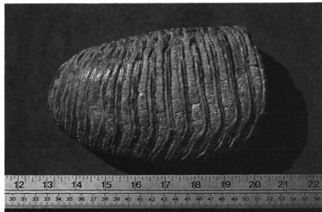
Figure 10 Waterworn partial mammoth ( Mammuthus primigenius ) tooth. Note cobbler-like form with transverse grinding ridges worn smooth within general outline and broken right margin. Late Pleistocene (probably Late Wisconsinan) gravels at West Peace River, Alberta. This specimen is in the Peace River Centennial Museum.
