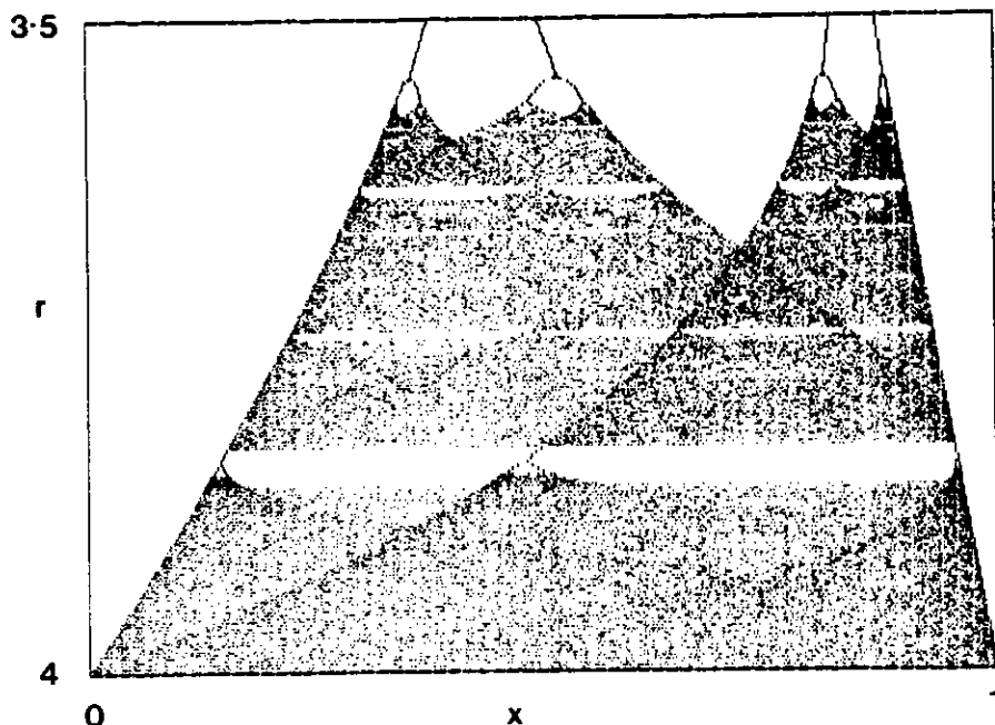
Figure 3 The Logistic Map. The map is shown for the range x = 0 to 1.0 , and r = 3.5 to 4.0 . The first bifurcation takes place at r = 3.0 , and the second at r = 3.45 . The chaotic region begins at r = 3.57 .
