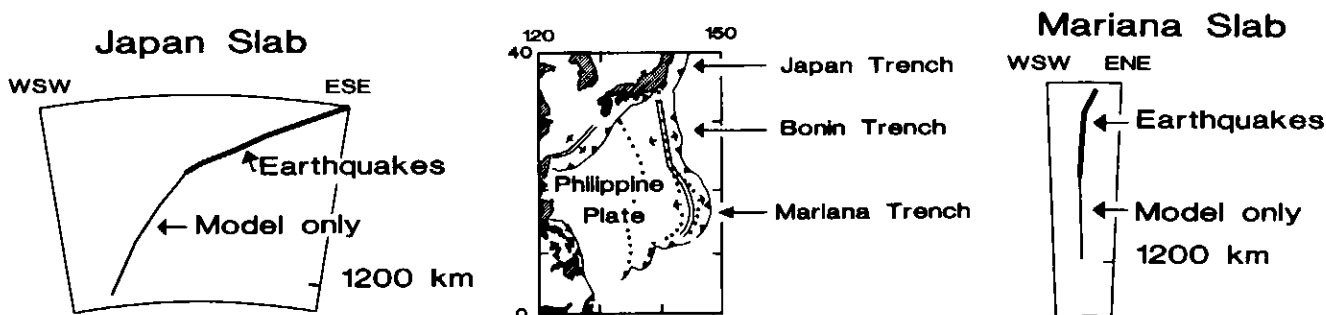
Figure 4 The Mariana and the Bonin Trenches are the eastern boundaries to the Philippine Plate.
