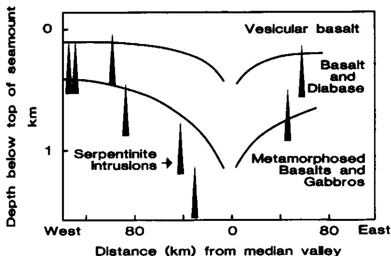
Figure 3 Serpentine intrusions appear to rise higher with distance from the axis of the Mid-Atlantic Ridge. The original caption read in part: "A plot of the depth below the top of the nearest seamount for those locations yielding serpentinite against distance from the axis of the Ridge. The plots are superimposed on the probable layering of the crust prior to block faulting as observed by Barrett and Aumento (1970)." (Redrawn from Aumento and Loubat, 1971, fig. 2).
