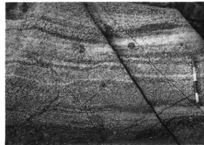
(c) Mafic cumulates, characterized by metamorphosed plagioclase- (light) and clinopyroxene-rich (dark) layers. Length of pen is 15 cm.
