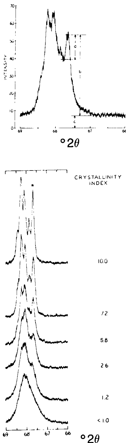
Figure 13 (a) X-ray diffractogram showing the quartz quintuplet at about 68^{\circ}2\theta , and the parameters a and b used to define the quartz crystallinity index CI of Murata and Norman (1976, fig. 2; for explanation see text). (b) Tracings of diffractograms showing increasing quartz crystallinity from bottom to top. Asterisk marks (212) peak at 67.74^{\circ}2\theta which is used for the determination of the index. \text{CuK}_{\alpha} radiation (from Murata and Norman, 1976, fig. 1).
