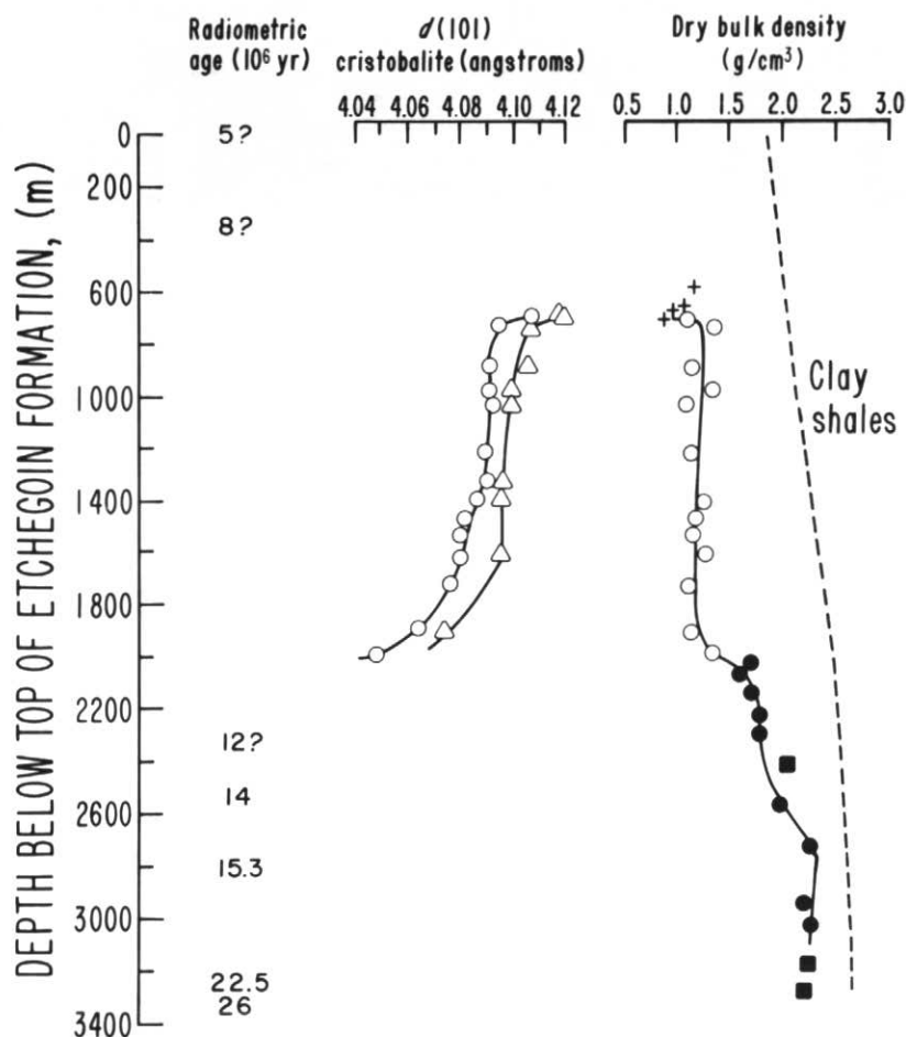
Figure 12 d(101) spacing of opal-CT in porcelainite (circles) and cherts (triangles) from the Monterey Formation in Chico Martinez Creek, plotted against depth below the top of the Etchegoin Formation (from Murata and Larson, 1975, fig. 6). Density data: crosses, diatomaceous shale; open circles, opal-CT porcelainite; half-filled circles, porcelainite with quartz; filled circles, quartz chert; filled squares, shale; dashed line, densities of normally compacting shales.
