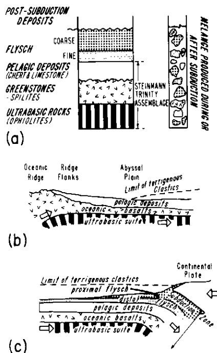
Figure 5 (a) Schematic representation of the "Steinmann trinity" (= ophiolite stratigraphy) of ultrabasic rocks, altered basalts and pelagic sediments (radiolarian cherts and limestones); (b) origin of the ophiolite stratigraphy through ocean crust generation at mid-oceanic ridges; and (c) its destruction in subduction zones (from Chipping, 1971).
