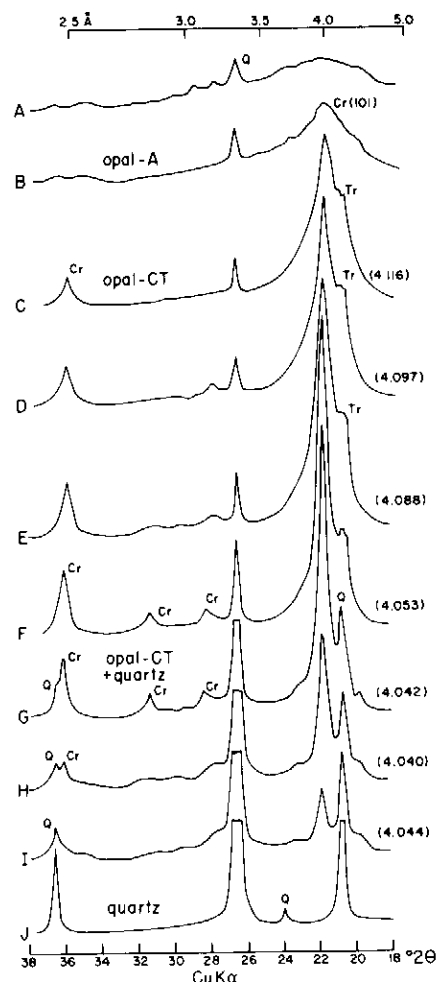
Figure 6 (A) X-ray diffractogram for opal-A (broad hump at about 4 Å) and detrital quartz (Q) in diatomaceous shale. (B to I) peak-sharpening and shift in position of the (101) diffraction of opal-CT with progressive burial in the Monterey Formation of California. Doublet peaks at 4.1 Å and 4.3 Å for cristobalite (Cr) and tridymite (Tr), respectively. Numbers in brackets: cristobalite-d(101) of opal-CT in angstroms. (J) Diffractogram of quartz chert. (Modified from Murata and Larson, 1975, fig. 5).
