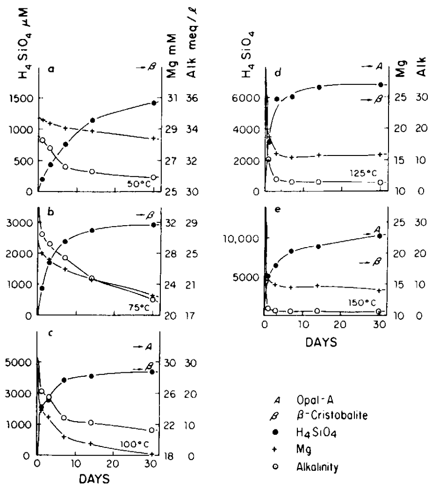
Figure 18 Changes in dissolved silicon, magnesium and alkalinity as a function of time and temperature in hydrothermal experiments with Eocene Radiolaria (specific surface area of 5.3 \text{ m}^2 \cdot \text{g}^{-1} ). \beta , solubility of \beta -cristobalite; \rightarrow A , solubility of opal-A (from Kastner and Gieskes, 1983, fig. 1).
