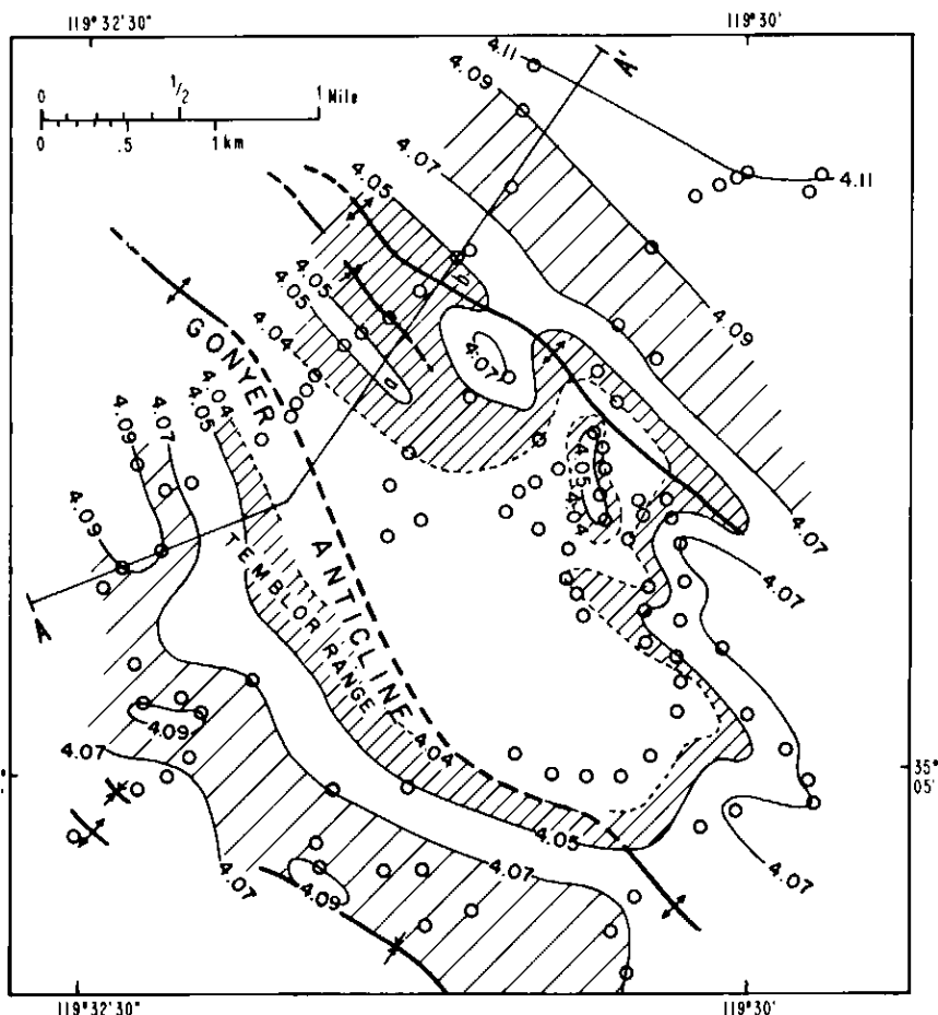
Figure 14 d(101) spacing isopleths for opal-CT porcelanite in the Temblor Range southwest of Taft (California). These provide an example of "isograd" mapping in low- to intermediate-grade diagenetic rocks. Note apparent congruency between structural features and diagenetic trends (Redrafted after Murata and Randall, 1975, fig. 4).
