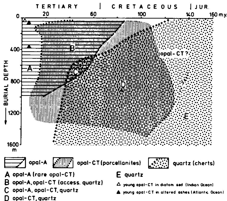
Figure 16 Age/burial fields for occurrences of opal-A, opal-CT and authigenic quartz in drill-holes of the Deep Sea Drilling Project (from v. Rad, 1979; after Riech and v. Rad, 1979).
