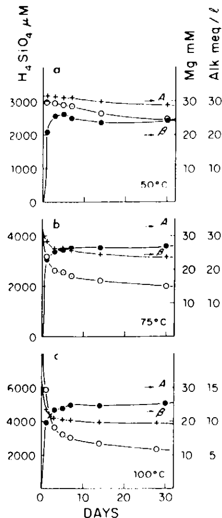
Figure 19 Changes as in Figure 18, however for Ludox silica (specific surface area of 61.5 \text{ m}^2 \cdot \text{g}^{-1} ; from Kastner and Gieskes, 1983, fig. 2).
