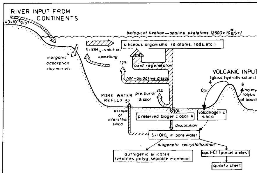
Figure 1 Global dissolved silicon budget of the oceans. (From Riech and v. Rad, 1979, modified after Heath, 1974). All numbers are in 10^{14} \text{ g SiO}_2 per annum
