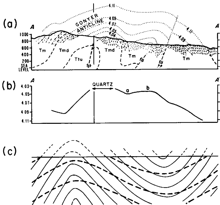
Figure 15 (a) Geologic cross-section with reconstructed d(101) spacing profiles for opal-CT in the Temblor Range showing near-concordant relationship between folding and maturation levels. For location of section A-A' see Figure 14. (Redrafted after Murata and Randall, 1975, fig. 5B).
