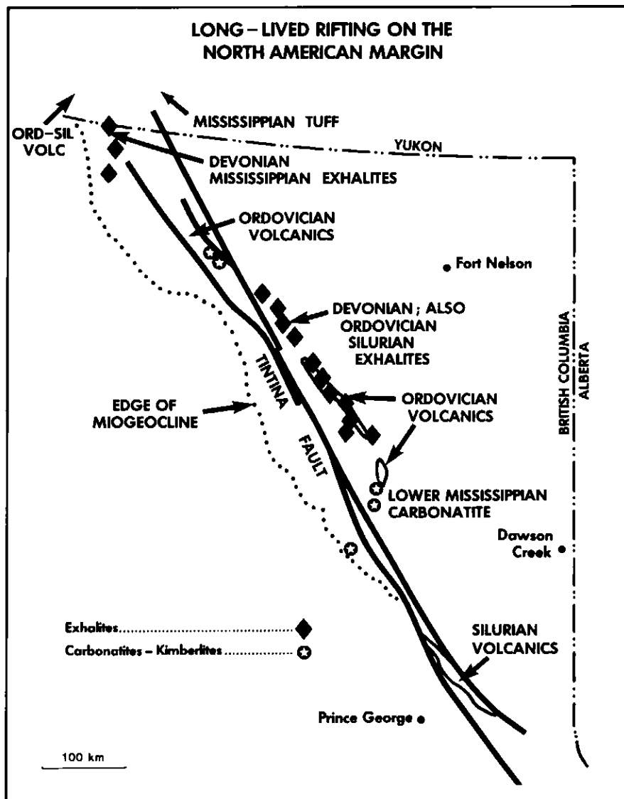
Figure 2 Evidence for long-lived, episodic Paleozoic rift activity on the North American continental margin.
