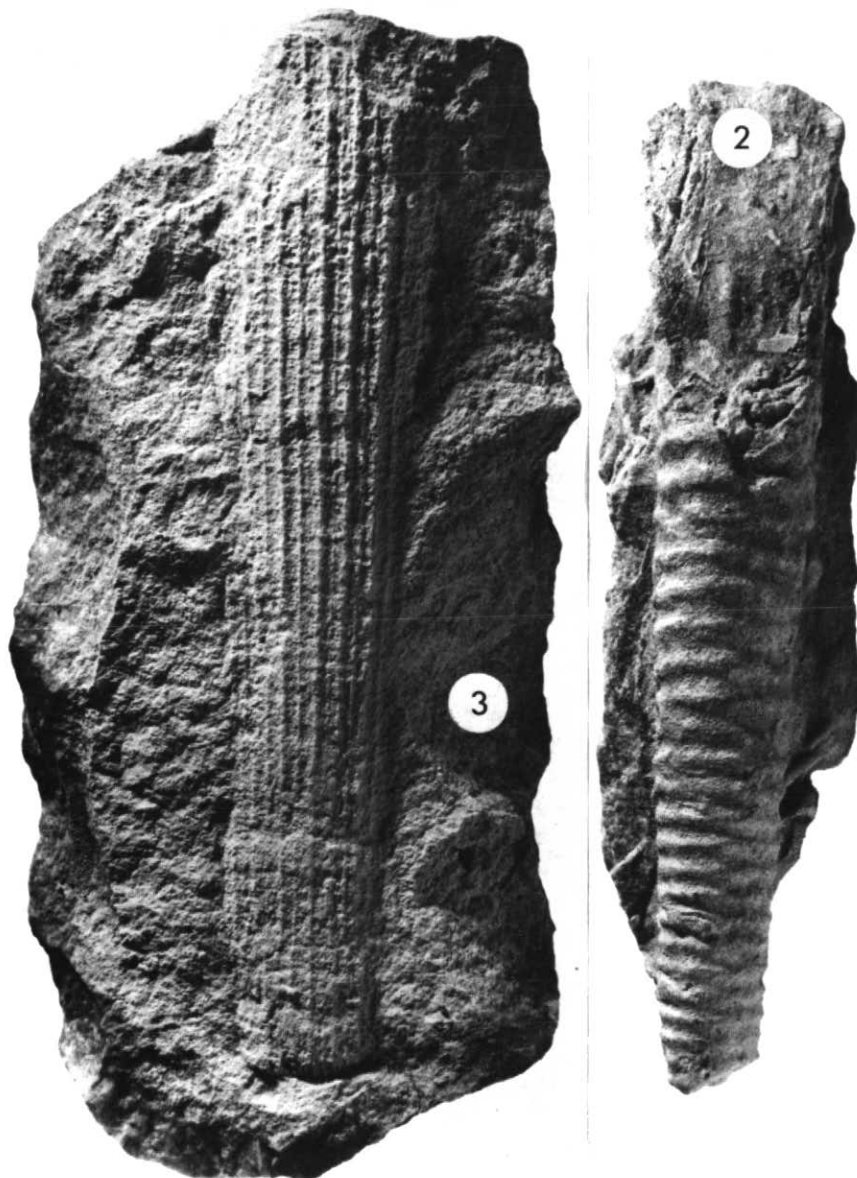
Figures 2 and 3 Bedding plane views of two orthocerid nautiloids collected by Grant at the Jolley Cut. Figure 2 is a ventral view of a cyrtconic mold of a Richmondian Gorbyoceras (length 140 mm). It was collected on the base of a thick sandstone bed, still seen 2.0 m above the base of the Whirlpool Sandstone. Labelled "RM 1108 Orthoceras sp. Medina — Hamilton, Ontario, Donor Col. Grant". Figure 3 shows a dolomite lithology from the base of a 0.4 m thick biostrome overlying the Gasport crinoidal facies. The 32-ribbed Kionoceras was figured by Grant (1910) as "no. 1" (S-319).
