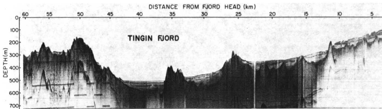
Figure 3 The effective sediment trap of a fjord as indicated on a 655 cm 2 airgun reflection-seismic profile.
