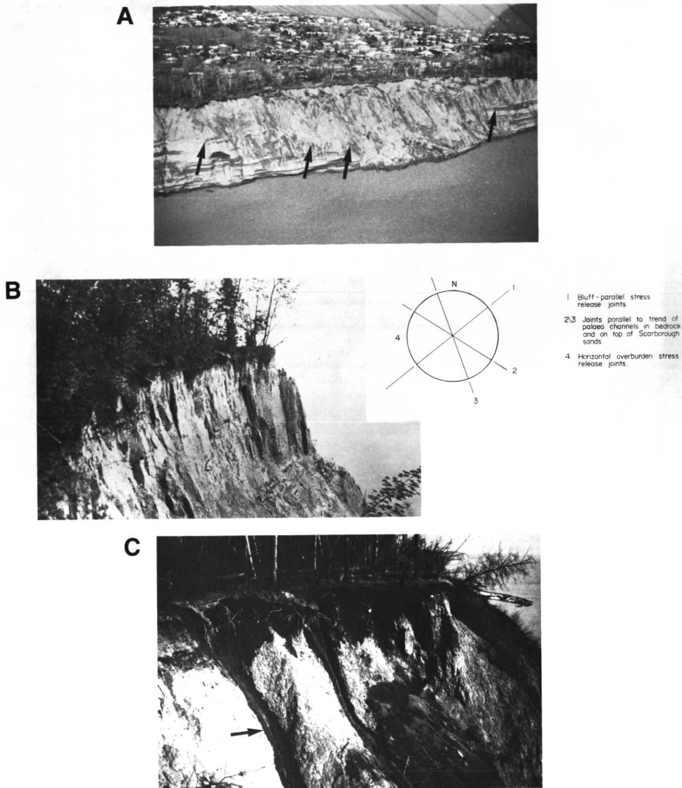
Figure 13 A) Air photograph of multiple shallow rotational failures involving diamict in the area of South Marine Drive. Sunnybrook diamict fills a paleochannel (arrowed) cut into the underlying Scarborough Sands (Fig. 3); B) Joint sets affecting Sunnybrook diamict and penetrating into underlying Scarborough Sands. Numbers refer to relative order of importance of joint sets in South Marine Drive area; C) Surface derived snow meltwater emerging under pressure (arrowed) from joints exposed along open bluff face (March 1985). Joint fed recharge to sands at the base of the paleochannel (Fig. 3) results in high porewater pressures particularly where free release of water is prevented by a mantle of slump debris. Periods of rotational slumping are observed to be associated with release of water from slope
