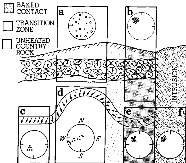
Figure 4 Stylized geological section showing examples of three basic field tests of magnetic stability: the conglomerate test (a, b), the fold test (c, d), and the baked-contact test (e, f). See text for details. The circles represent stereo-
