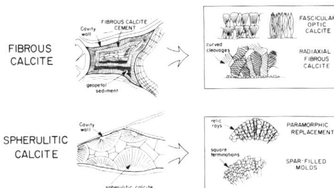
Figure 16 Fabrics and morphologies of coarse marine cements. Fibrous calcite is generally
