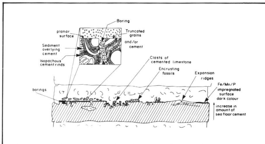
Figure 12 Criteria for the recognition of seafloor cementation.
