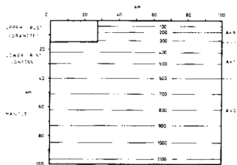
Figure 1a Dimensions and physical parameters of the two-dimensional burial and intrusion models. As the problem is symmetrical, only half of the model is shown. Thickness of the sediment or intrusion (stippled region) = 15 km, half-width = 27.5 km. Surrounding terrain is initially at its equilibrium thermal gradient. Deep heat contribution q_m = 0.5 \text{ h.f.u.} A = radioactive heat generation in h.g.u. For the burial model, initial temperature of the sediments is taken arbitrarily as 100^\circ\text{C} and A = 2 \text{ h.g.u.} In the basic intrusion, initial temperature = 1100^\circ\text{C} and A = 1 \text{ h.g.u.} In the granitic intrusion, initial temperature = 700^\circ\text{C} and A = 10 \text{ h.g.u.}
