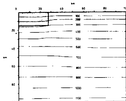
2b Basic intrusion after 20 Ma.
