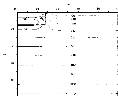
2c Granitic intrusion after 1 Ma.
