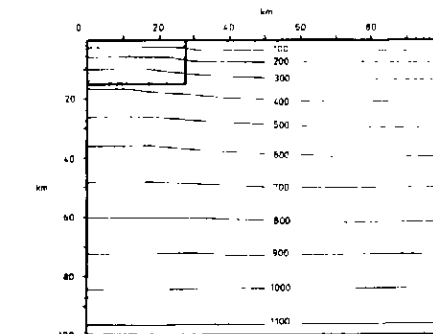
2f Granitic intrusion after 20 Ma.
