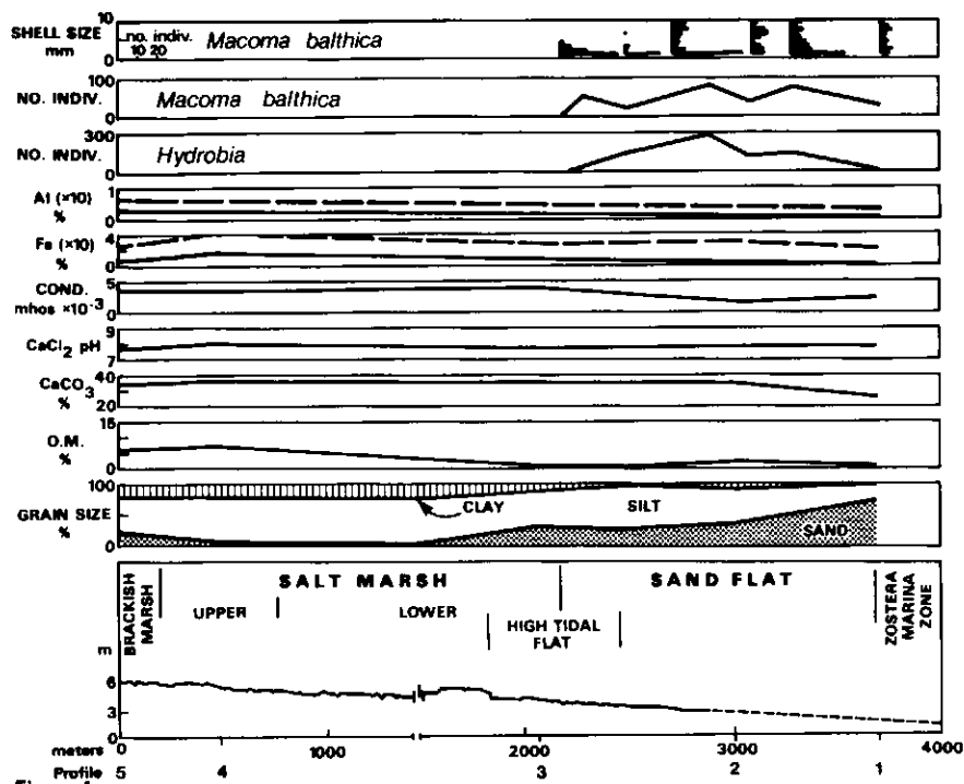
Figure 4 Lateral variations in environmental parameters measured on surface samples of BPE transect. Dashed lines indicate iron and aluminum values obtained from \text{NH}_4 -oxalate extract, solid lines
