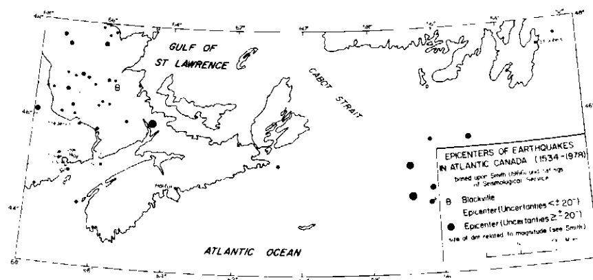
Figure 3 Earthquakes in Atlantic Canada
