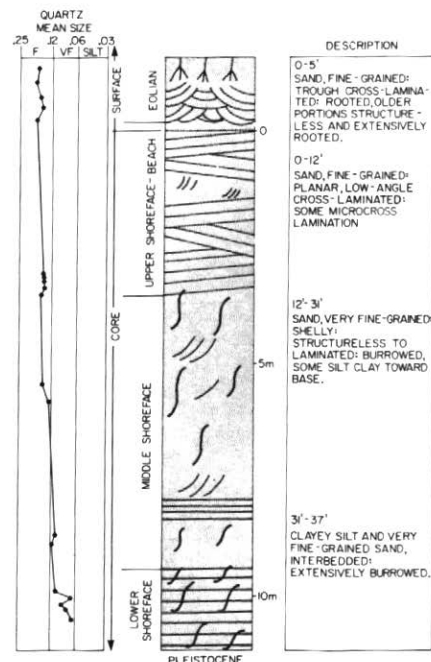
Figure 10 Sequence of sedimentary structures, textures and lithology in a core through Galveston Island (From Davies et al., 1971, Fig. 6).
